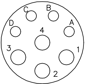
8 PIN MOTOR CONNECTOR THREADED CRIMP PIN STYLE
