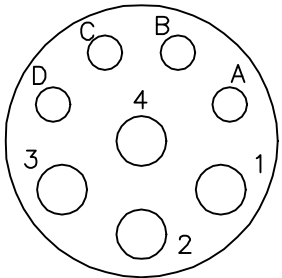
8 PIN MOTOR CONNECTOR THREADED CRIMP PIN STYLE
