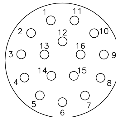
16 PIN CONNECTOR THREADED CRIMP PIN STYLE
