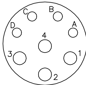
8 PIN THREADED CONNECTOR (CRIMP STYLE) (INSERTION SIDE)
