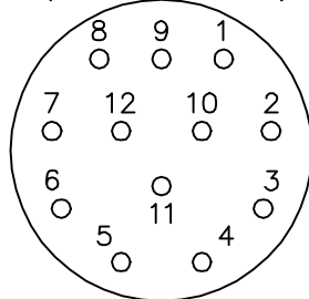
12 PIN THREADED CONNECTOR (CRIMP STYLE) (INSERTION SIDE)
