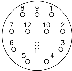
12 PIN THREADED CONNECTOR (INSERTION SIDE)
