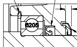
PULLEY END DETAIL
