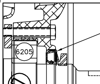
PULLEY END DETAIL
