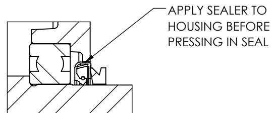
PULLEY END DETAIL
