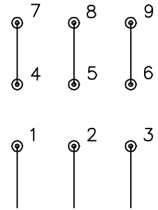
HIGH VOLTAGE (1D)
