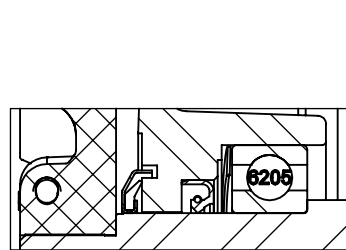
FRONT END DETAIL
