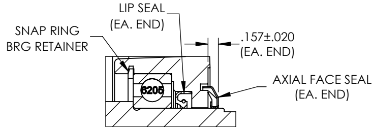
PULLEY END DETAIL
