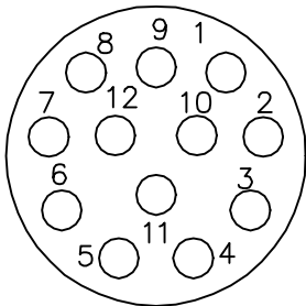
12 PIN THREADED CONNECTOR (CRIMP STYLE) (INSERTION SIDE)
