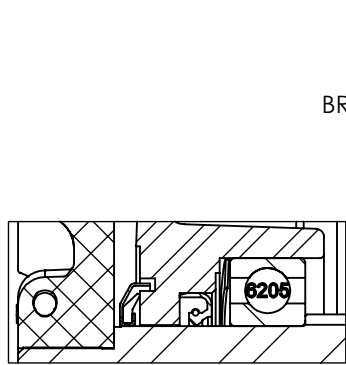
FRONT END DETAIL
