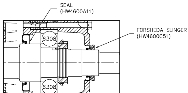
PULLEY DETAIL
