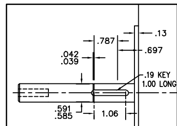
FR END SHAFT DETAIL
