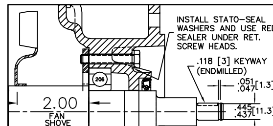
PULLEY END DETAIL
