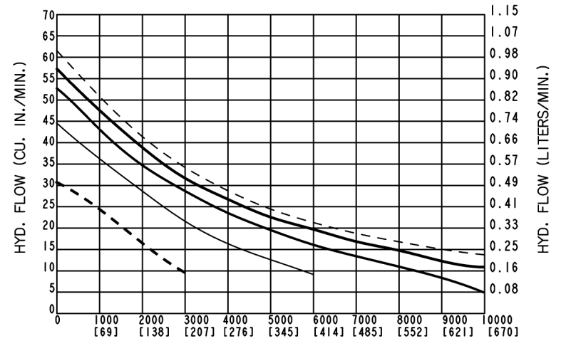
10,000 PSI PATG SERIES PERFORMANCE OF HYD. FLOW VS HYD. PRESSURE
