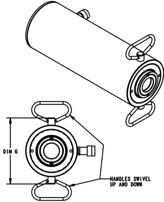
RACH 60/100/150 SERIES SCALE 1:4
