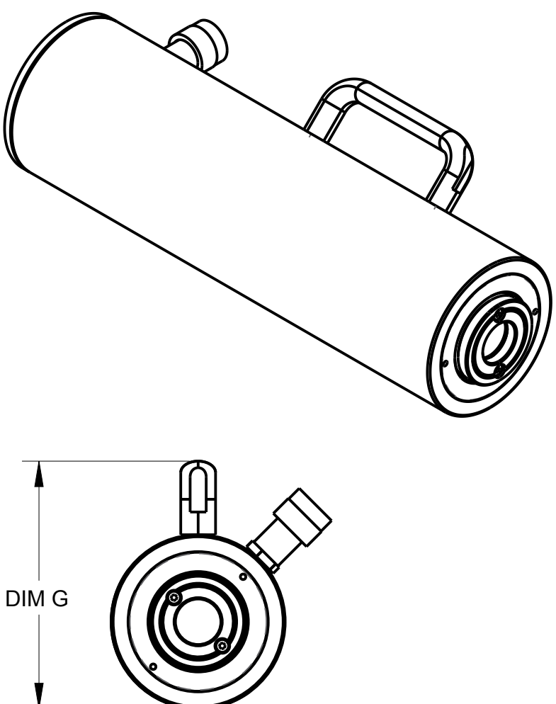
RACH 30 SERIES SCALE 1:4
