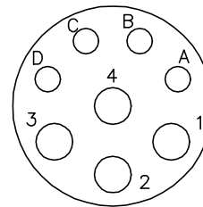
8 PIN MOTOR CONNECTOR THREADED CRIMP PIN STYLE
