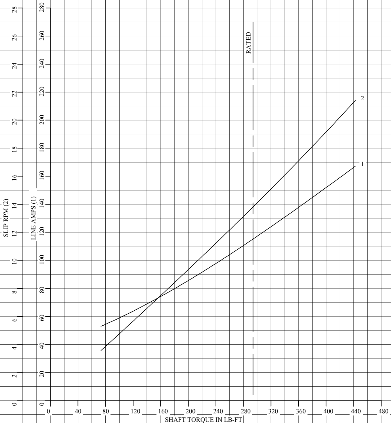
VECTOR PWM INVERTER DUTY LOAD PERFORMANCE (CONSTANT V/HZ RANGE)
