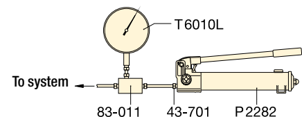
▲ Typical Test System
