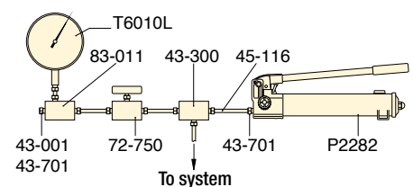
▲ Test System with Gauge and Snubber
