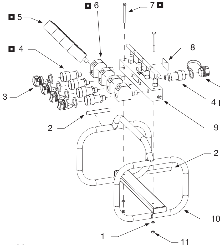
Fig. 1, AMGC41 ASSEMBLY
