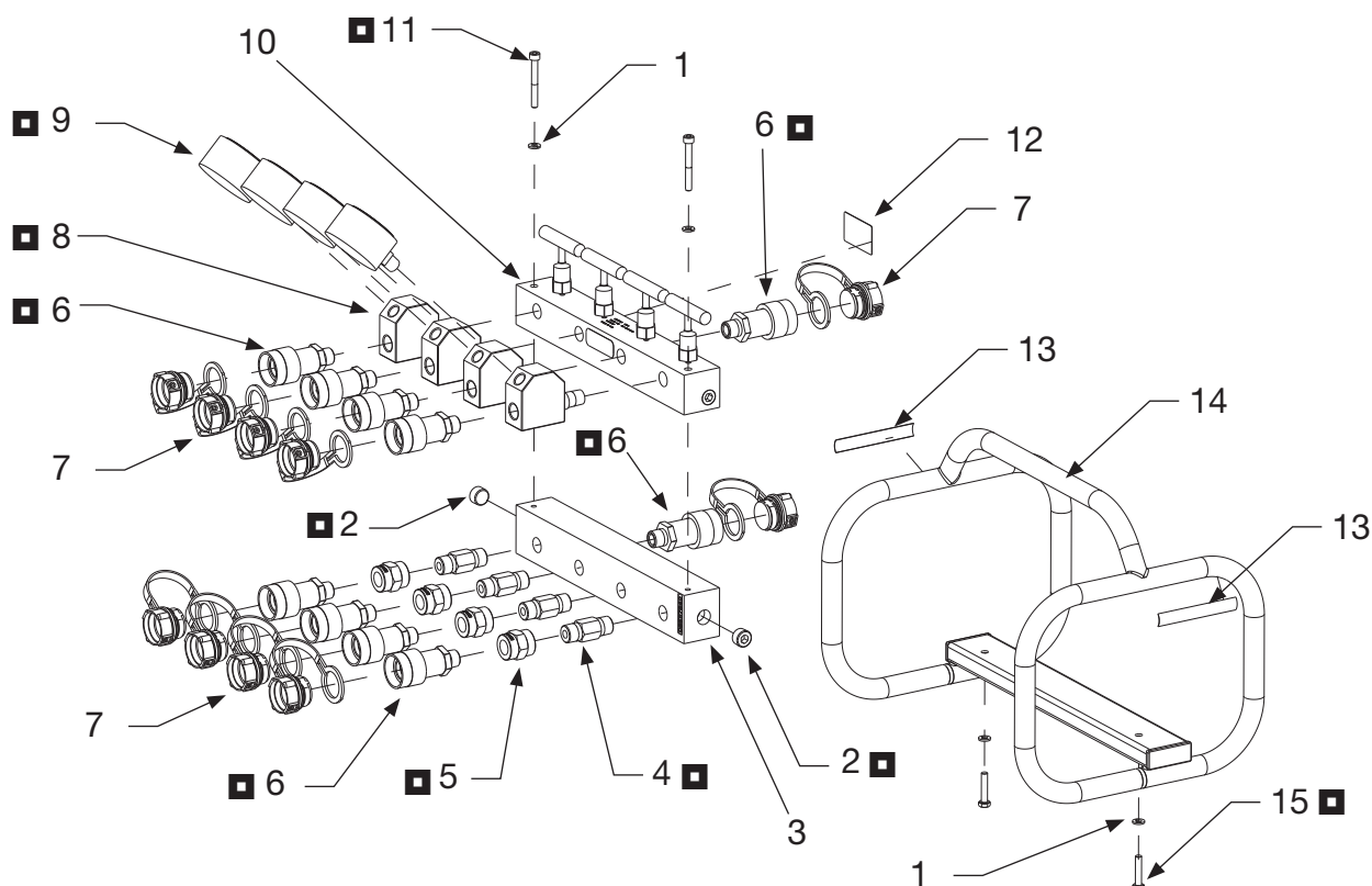
Fig. 2, AMGC42 ASSEMBLY
