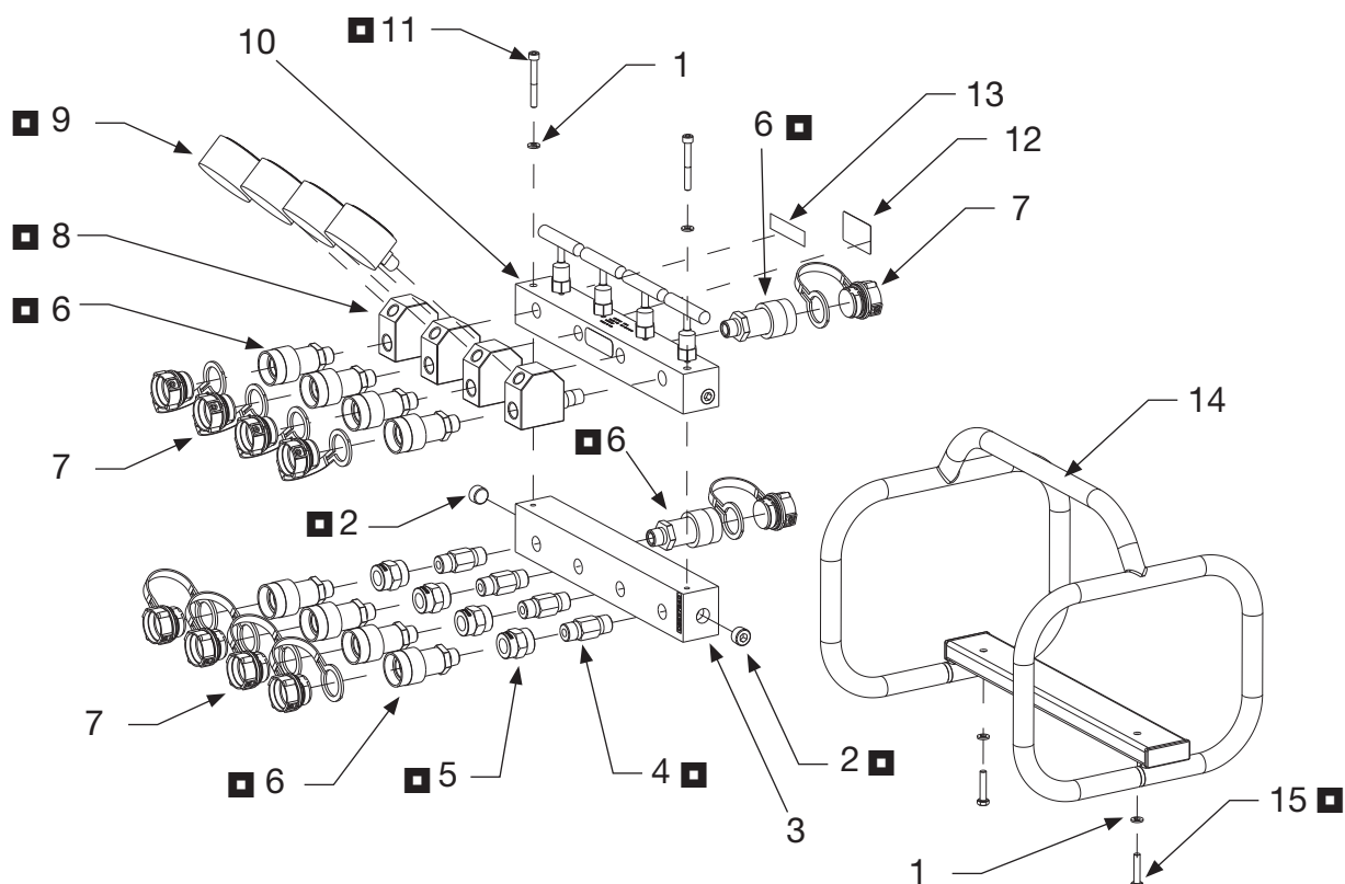
Fig. 2, AMGC42 ASSEMBLY
