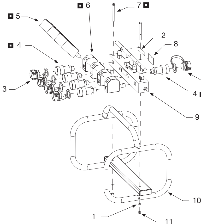
Fig. 1, AMGC41 ASSEMBLY
