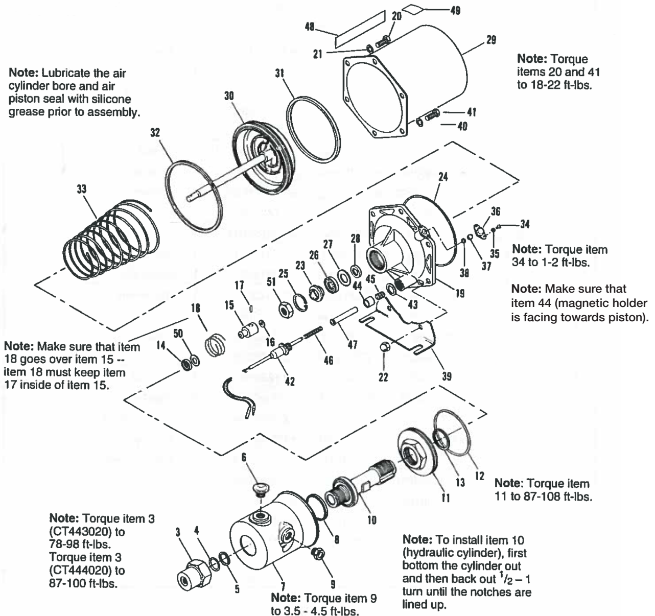
Figure 1, Hydraulic Boosters
