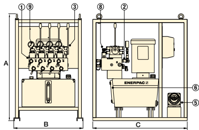
SFP-Series with 40-litre reservoir (shown with 4 split-flow outlets)
