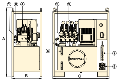
SFP-Series with 135-litre reservoir (shown with 4 split-flow outlets)
