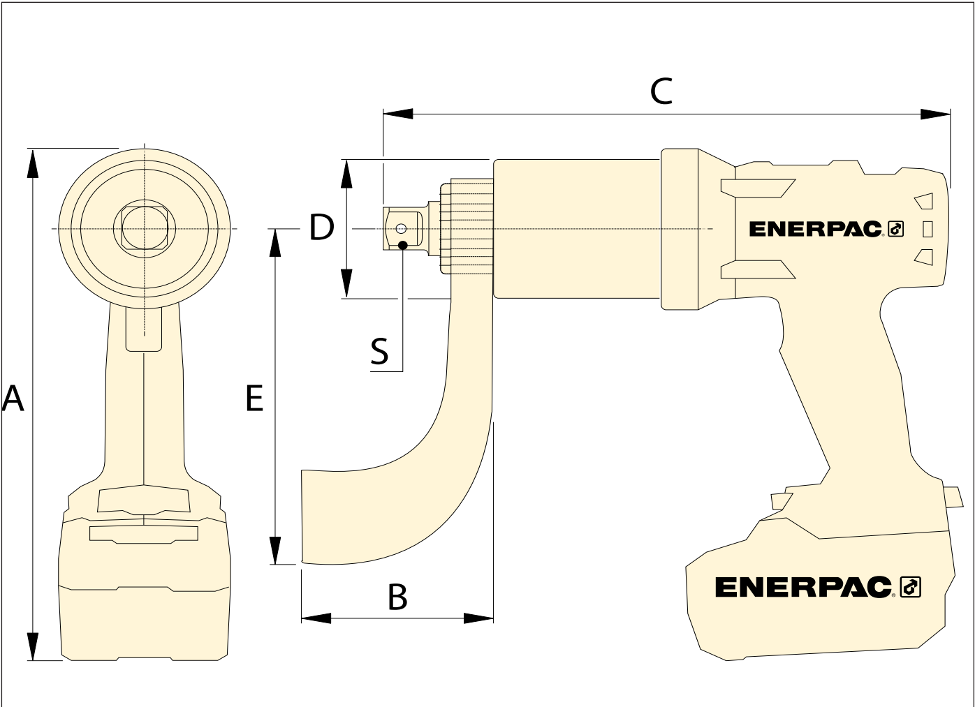
Figure 1: Dimensions
