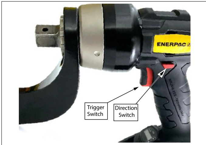
Figure 5: Trigger Switch
