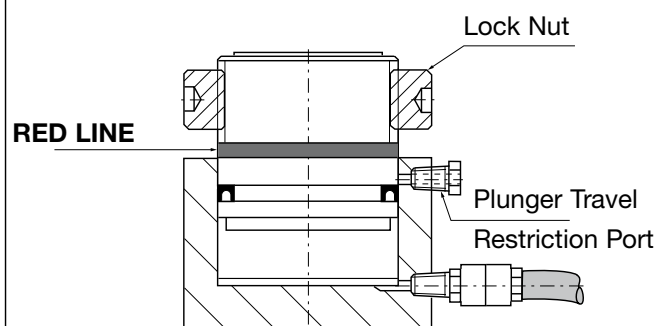
Illustration 1 - CLP cylinders
