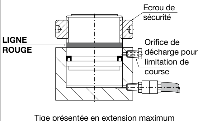
Illustration 1 - vérins CLP
