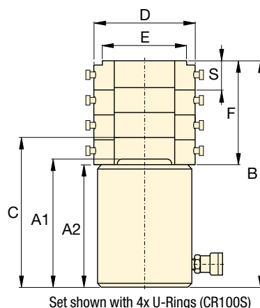
Set shown with 4x U-Rings (CR100S)
