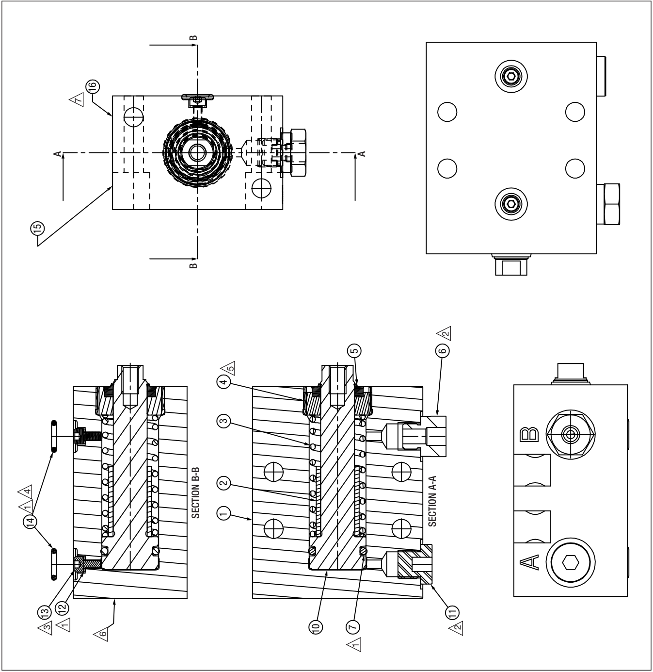
Figure 1: Cylinder Assembly - CSB Series
