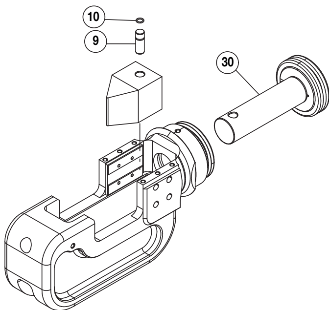
Figure 6 - ECCE3203K Piston Kit
