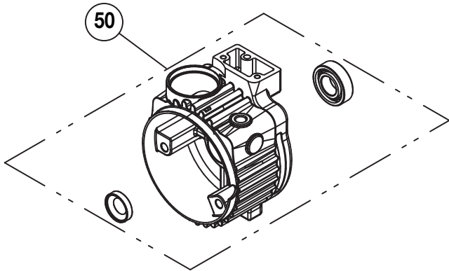
Figure 12 - ECCE3212K Tank Kit
