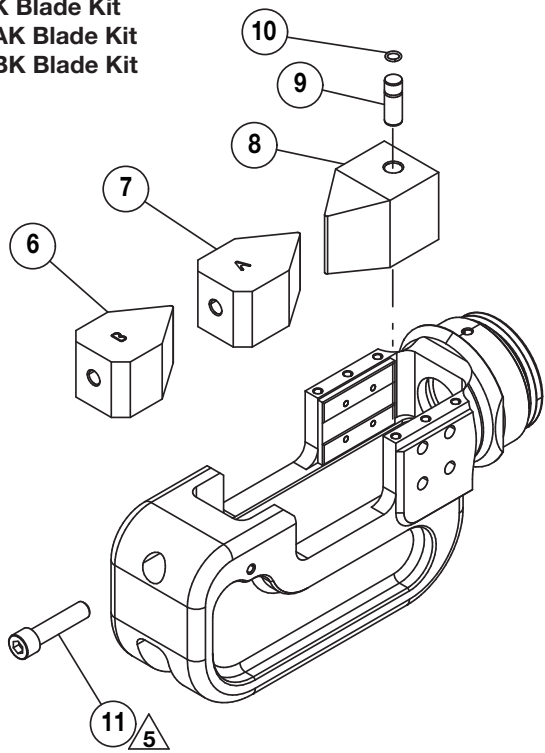
Figure 2 - Blade Kits
