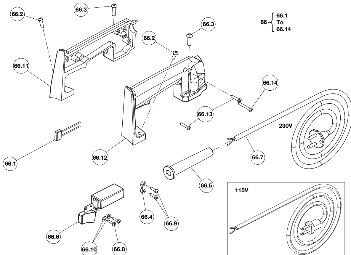
Figure 14 - EBE2219K & EBE2204K Handle Kit
