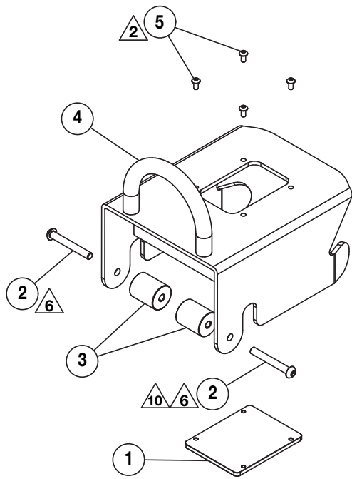
Figure 3 - ECCE3202K Guard Kit
