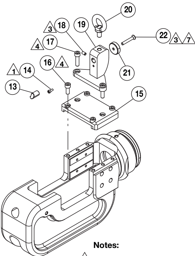
Figure 5 - ECCE3204K Top Cover Kit
