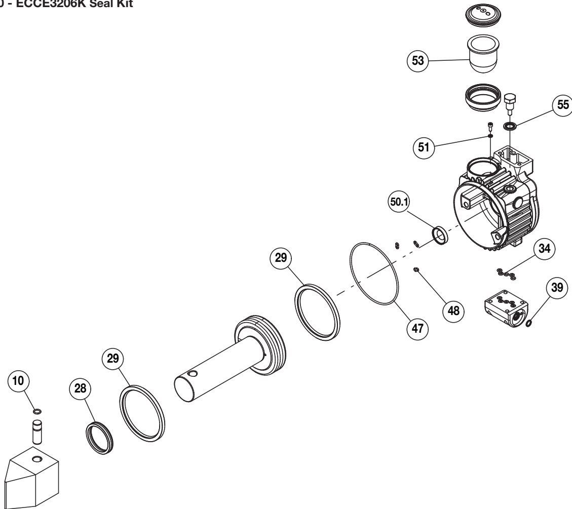
Figure 10 - ECCE3206K Seal Kit
