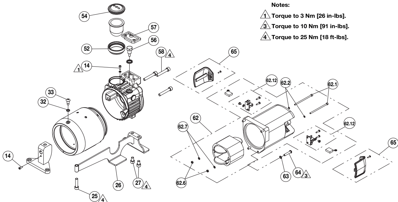
Figure 21 - ECCE3213K Small Parts Kit
