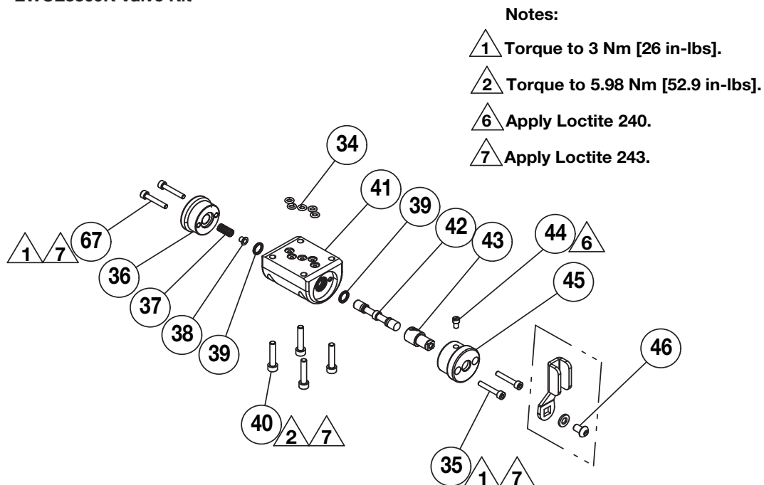
Figure 20 - EWCE5509K Valve Kit
