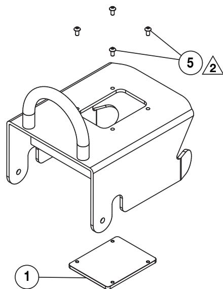
Figure 7 - ECCE2606K Guard Window Kit
