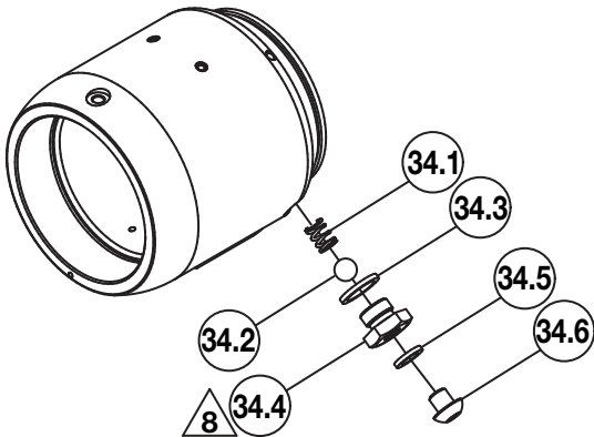
Figure 13- ECCE3209K Gauge Port Kit
