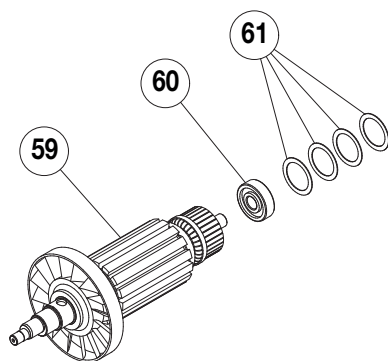
Figure 17 - EBE2211K & EBE2220K Rotor Kit
