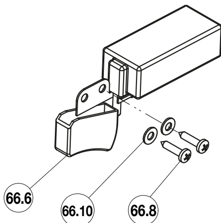
Figure 15 - EBE2223K & EBE2203K Switch Kit
