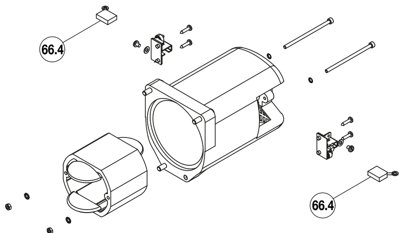
Figure 18 - EBE2222K and EBE2215K Brush Kit
