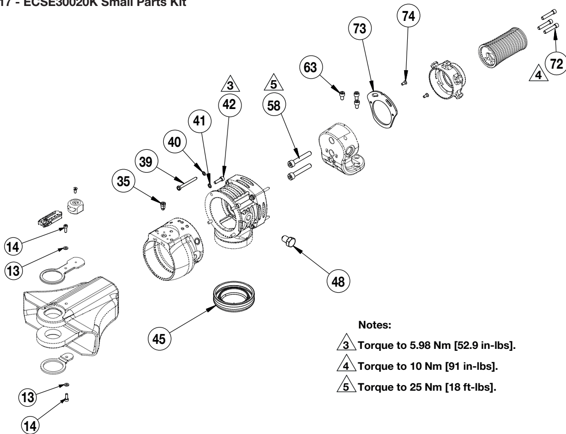
Figure 17 - ECSE30020K Small Parts Kit
