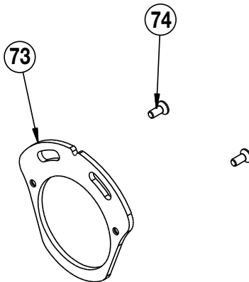
Figure 18 - ECSE30022K Valve Grip Guard Kit
