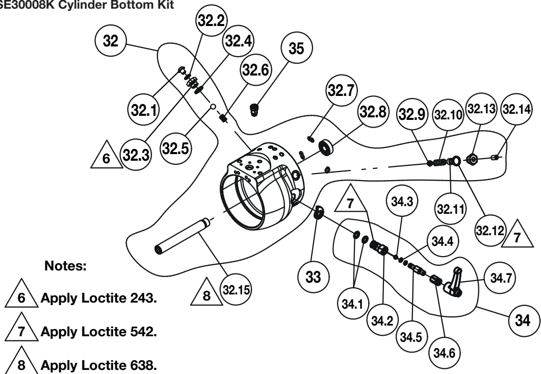
Figure 9 - ECSE30008K Cylinder Bottom Kit
