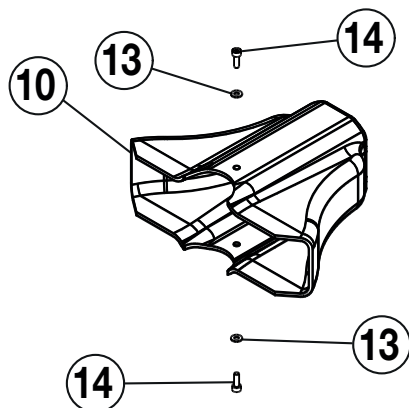
Figure 6 - ECSE30003K Cover Kit
