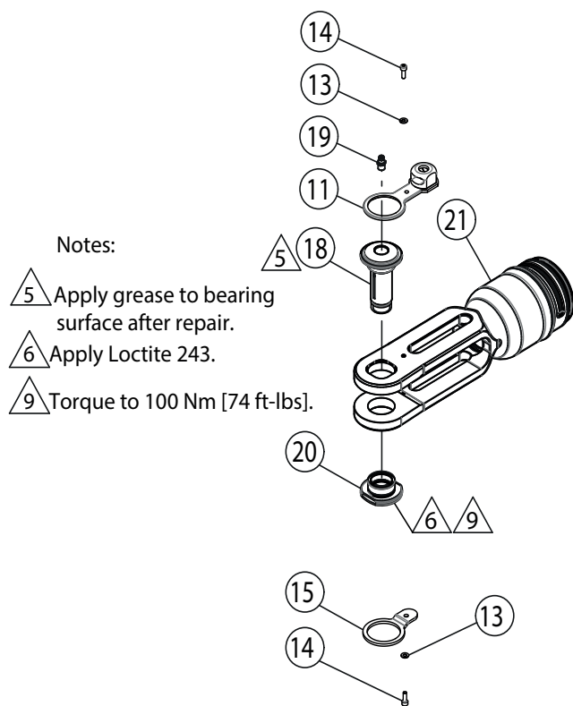
Figure 5 - ECSE30005K Cylinder Body Kit
