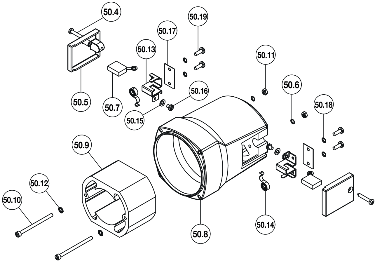
Figure 23 - ECCE2615K & ECCE2621K Motor Kit
