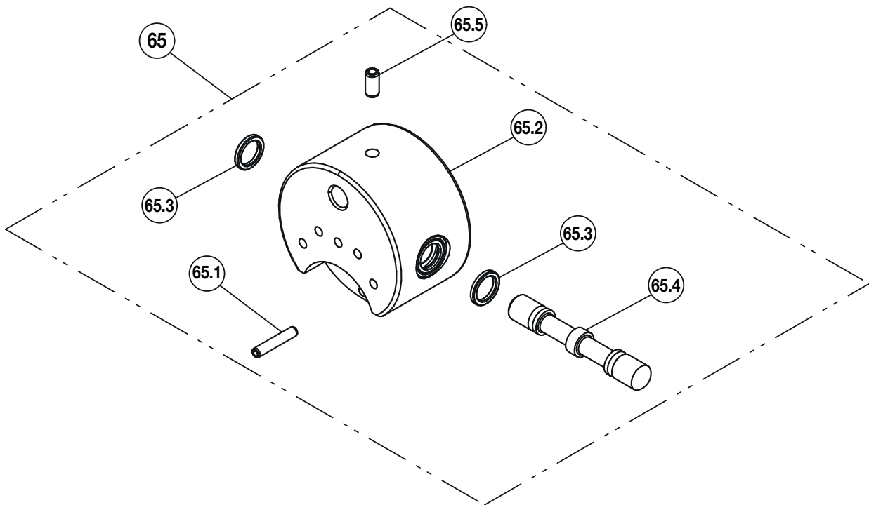
Figure 20 - ECSE30010K Distributor Kit
