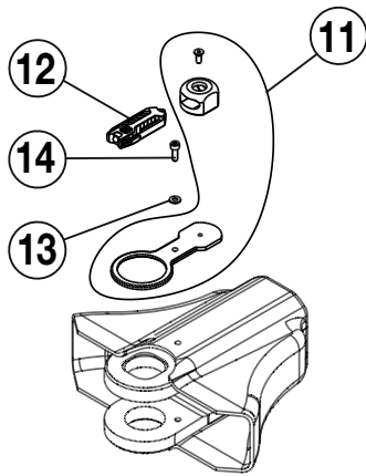
Figure 7 - ECSE30004K Light Kit
