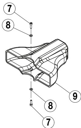
Figure 5 - EDCH13003K Cover Kit
