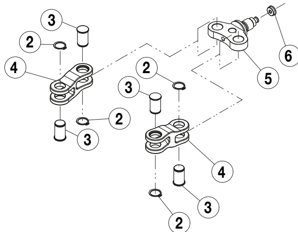
Figure 4 - EDCH13002K Linkage Kit
