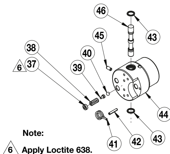
Figure 14 - EDCH13012K Rear Valve Kit
