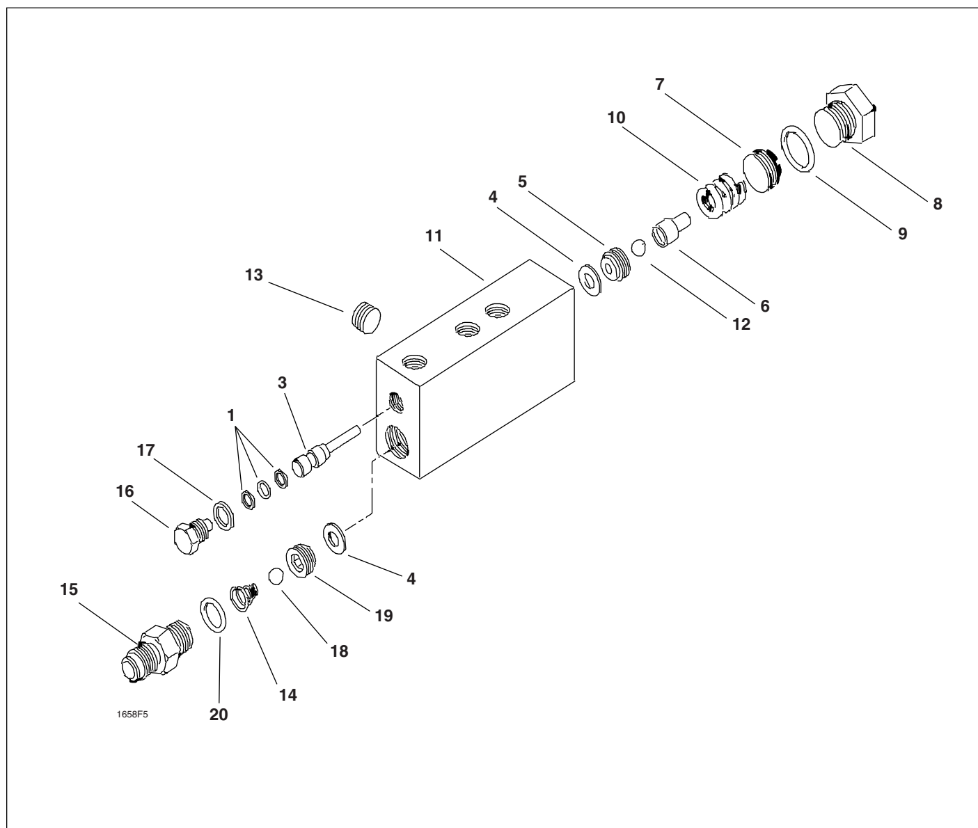
Figure 10, CU316900 By-pass Valve
