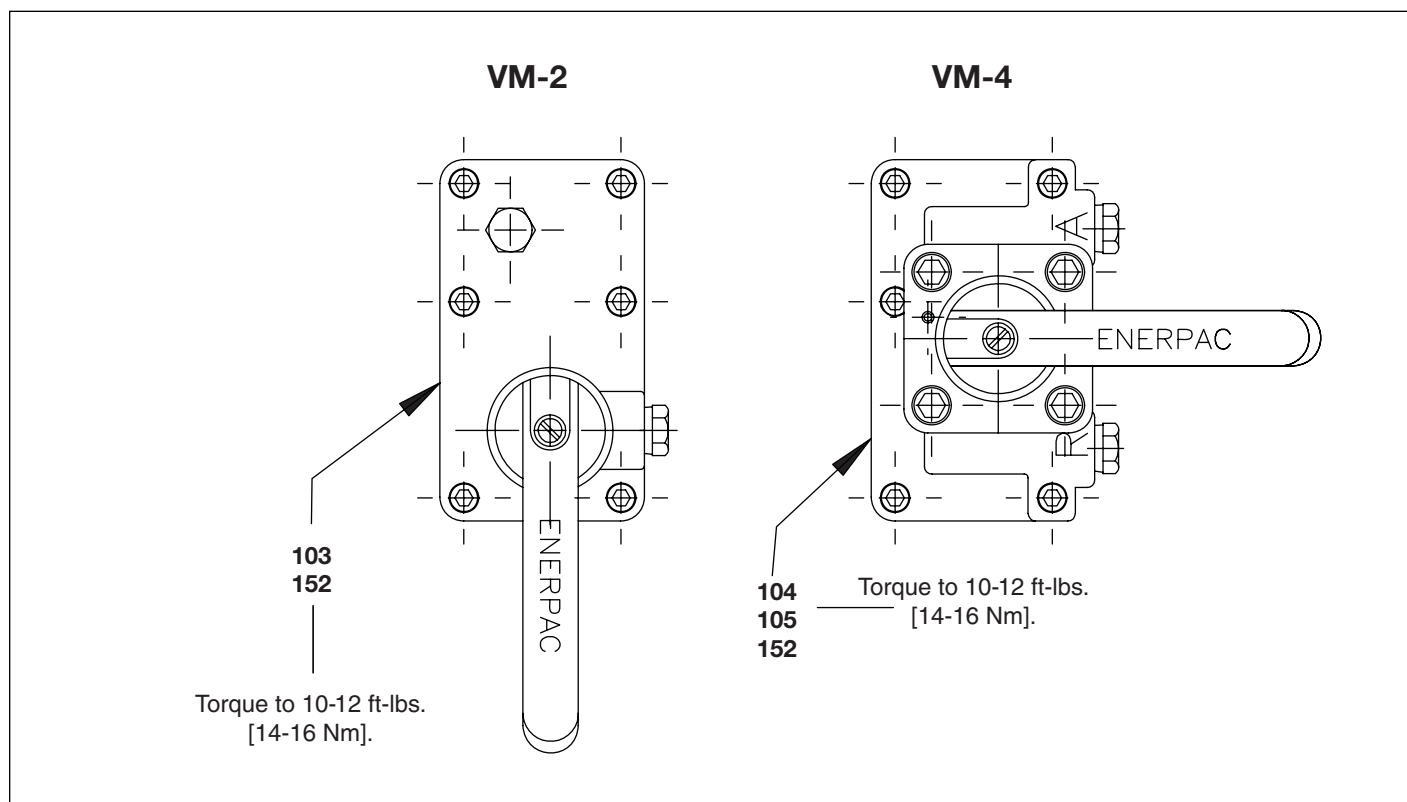
Figure 4, Manual Valve
