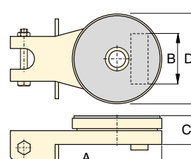
ES10, ES15, ES30 Turntable Swivel
