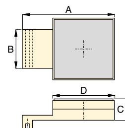
ELP60, ELP80 Levelling Plate
