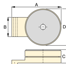
ES60, ES80 , Turntable Swivel
