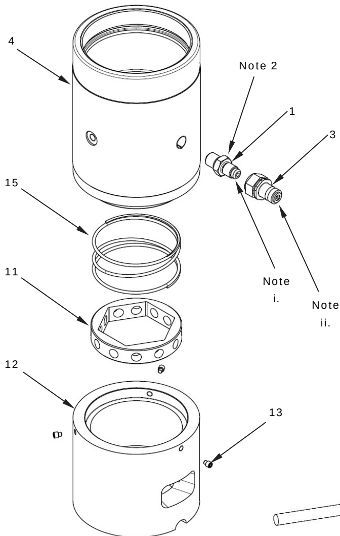
Figure 1, Exploded View, FTR-Series Foundation Tensioners, Round
