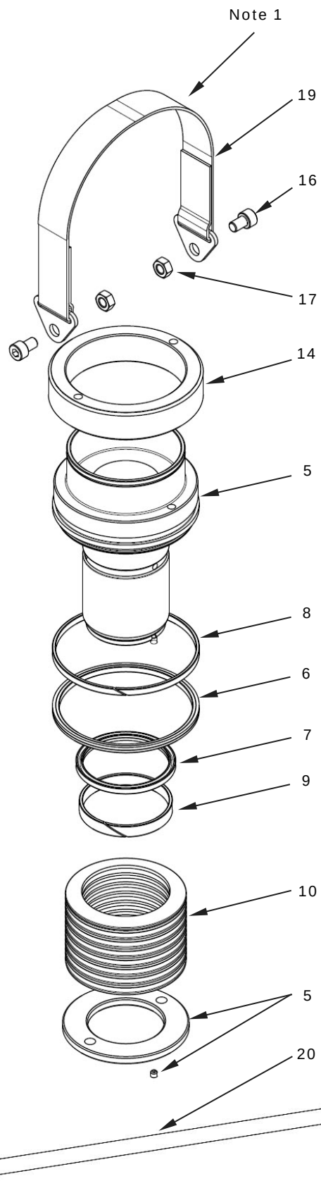
Figure 1, Exploded View, FTR-Series Foundation Tensioners, Round
