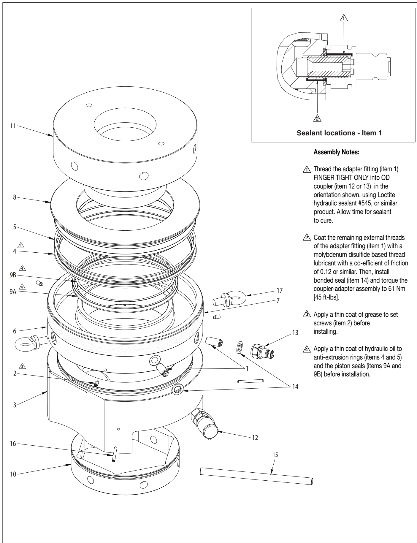
Figure 3, Exploded View, GT Series Hydraulic Tensioner (Models GT7)
