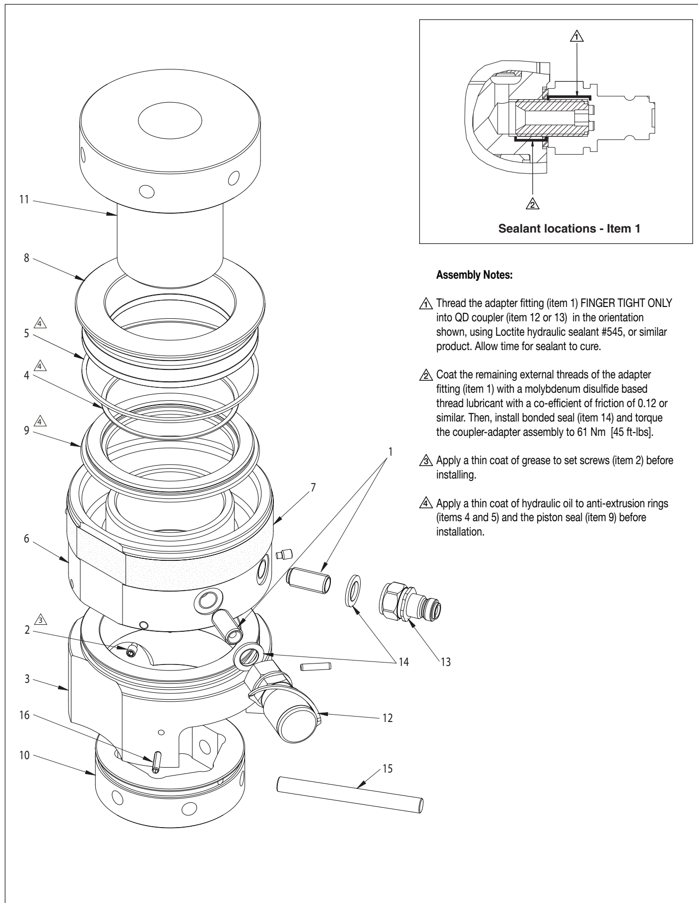
Figure 1, Exploded View, GT Series Hydraulic Tensioner (Models GT1, GT2 and GT3)
