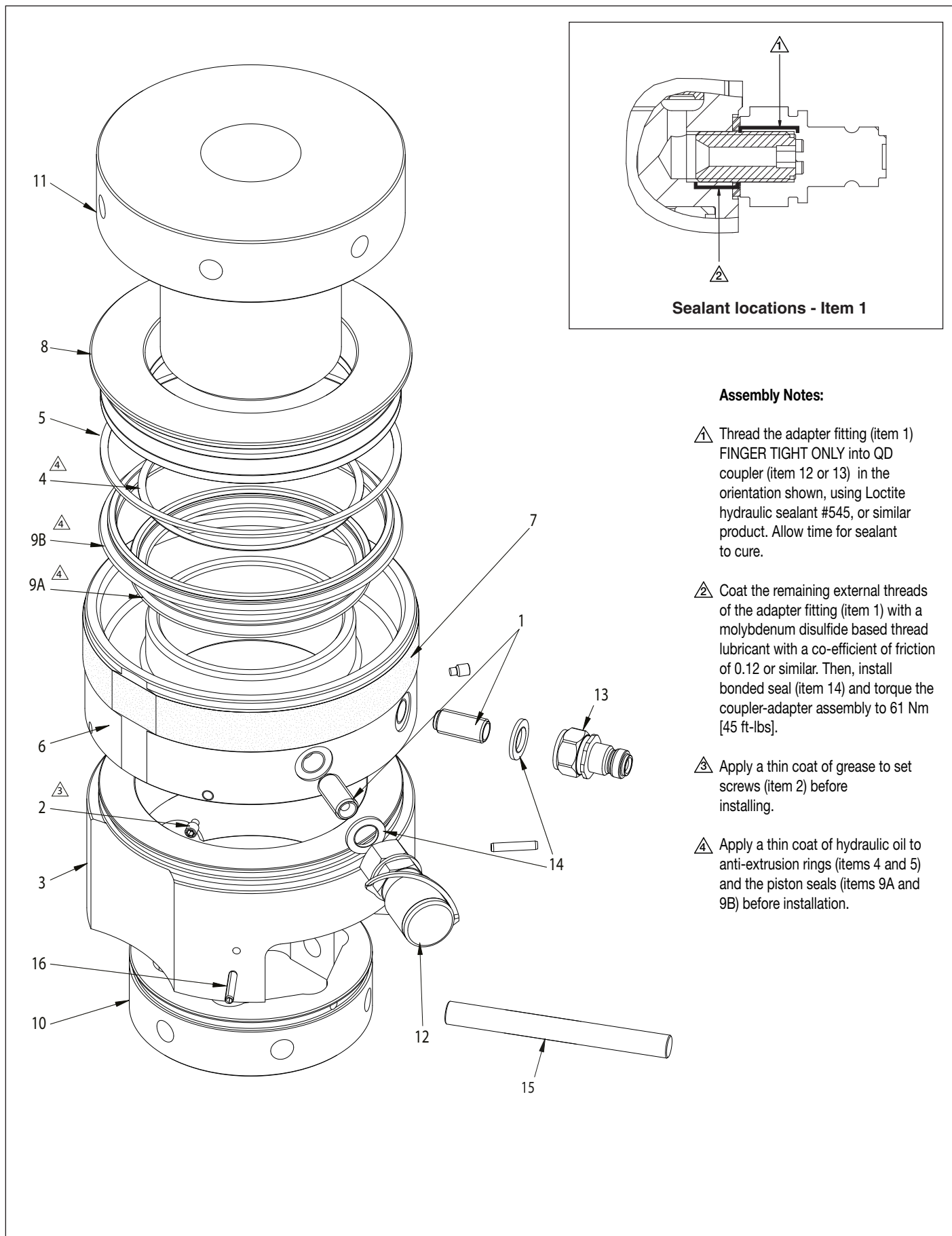
Figure 2, Exploded View, GT Series Hydraulic Tensioner (Models GT4, GT5 and GT6)
