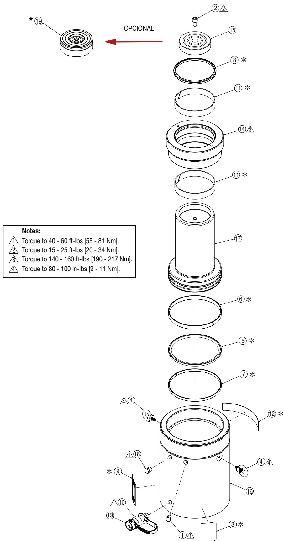
Figure 3, Exploded View - Model HCG-200 Short
