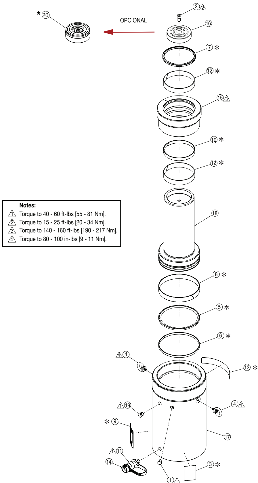
Figure 4, Exploded View - Model HCG-200 Tall
