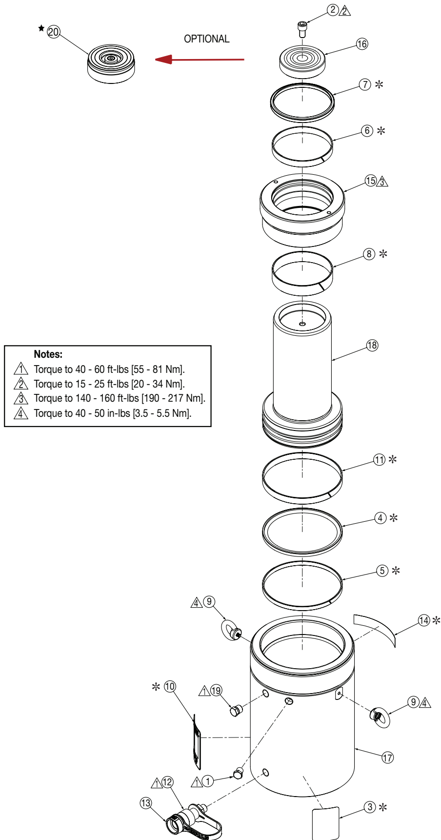
Figure 1, Exploded View - Model HCG-150 Short
