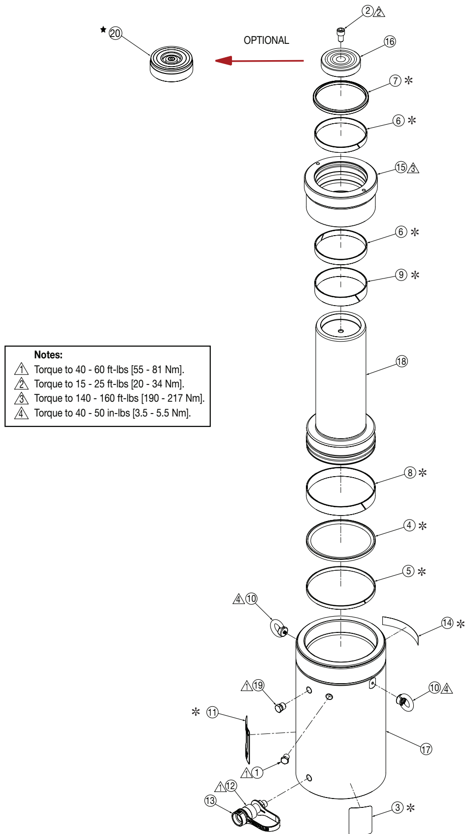
Figure 2, Exploded View - Model HCG-150 Tall
