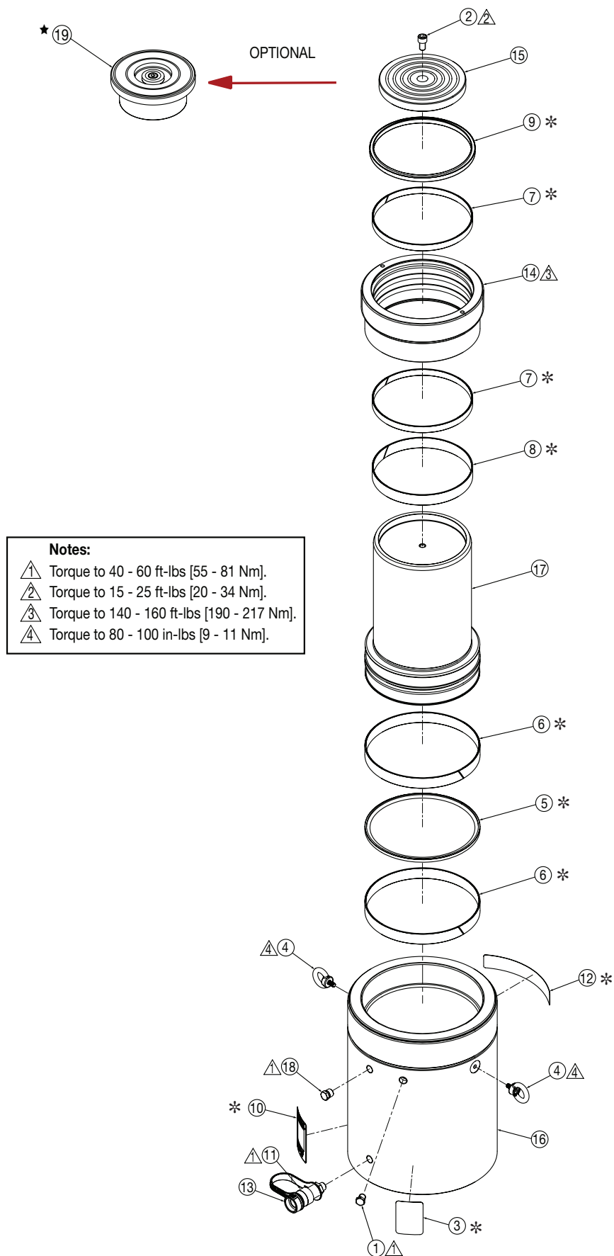
Figure 3, Exploded View - Model HCG-300
