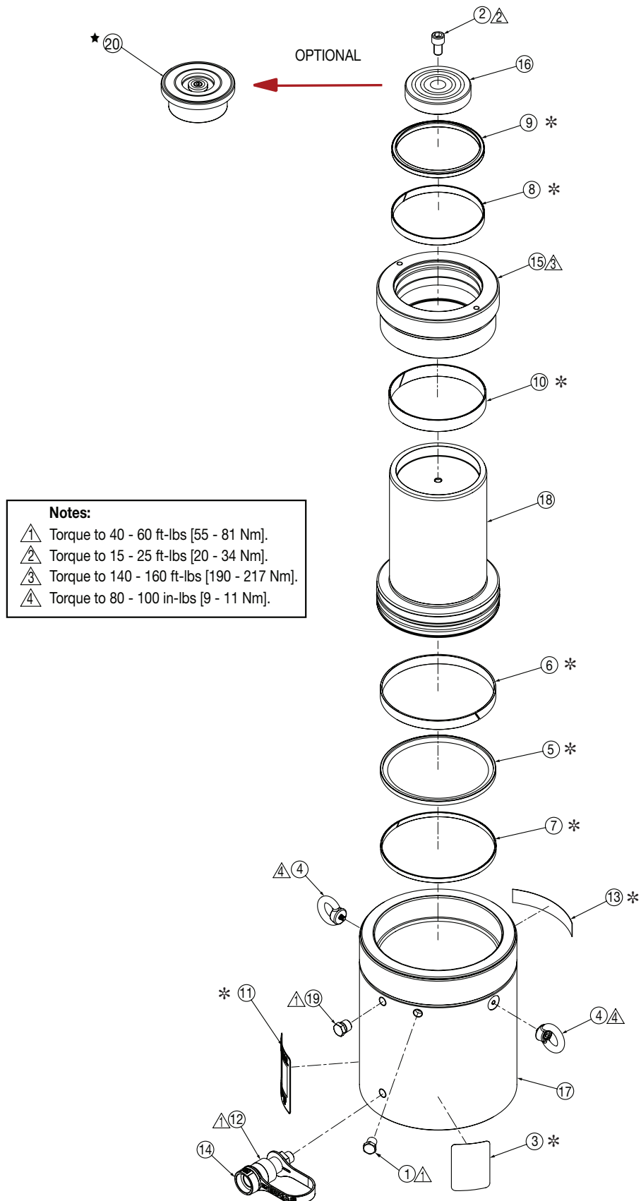
Figure 1, Exploded View - Model HCG-250 Short
