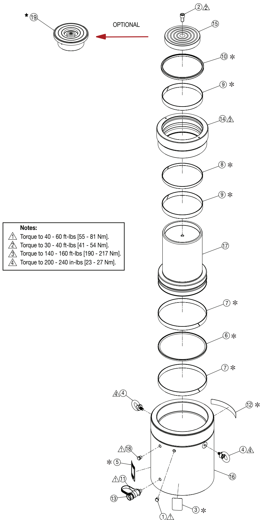
Figure 4, Exploded View - Model HCG-400
