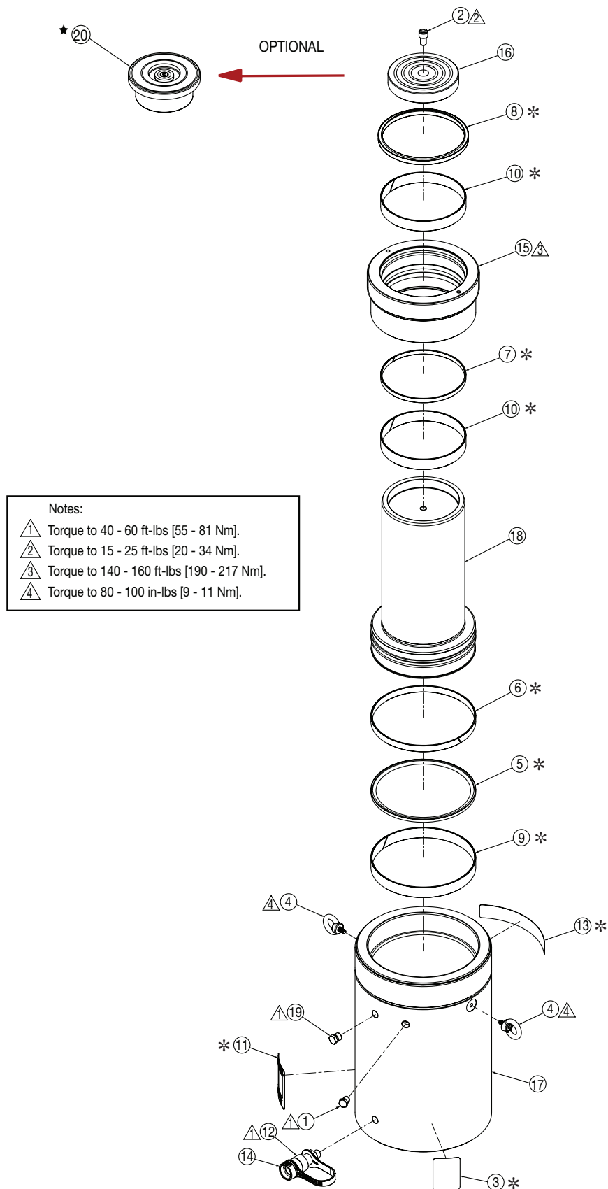
Figure 2, Exploded View - Model HCG-250 Tall
