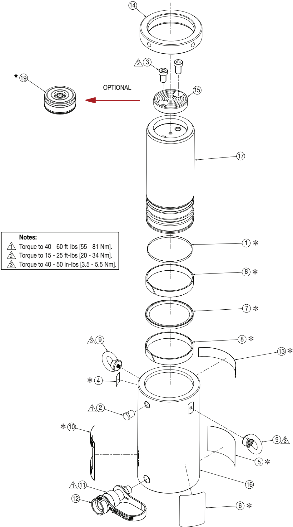
Figure 1, Exploded View - Model HCL-50
