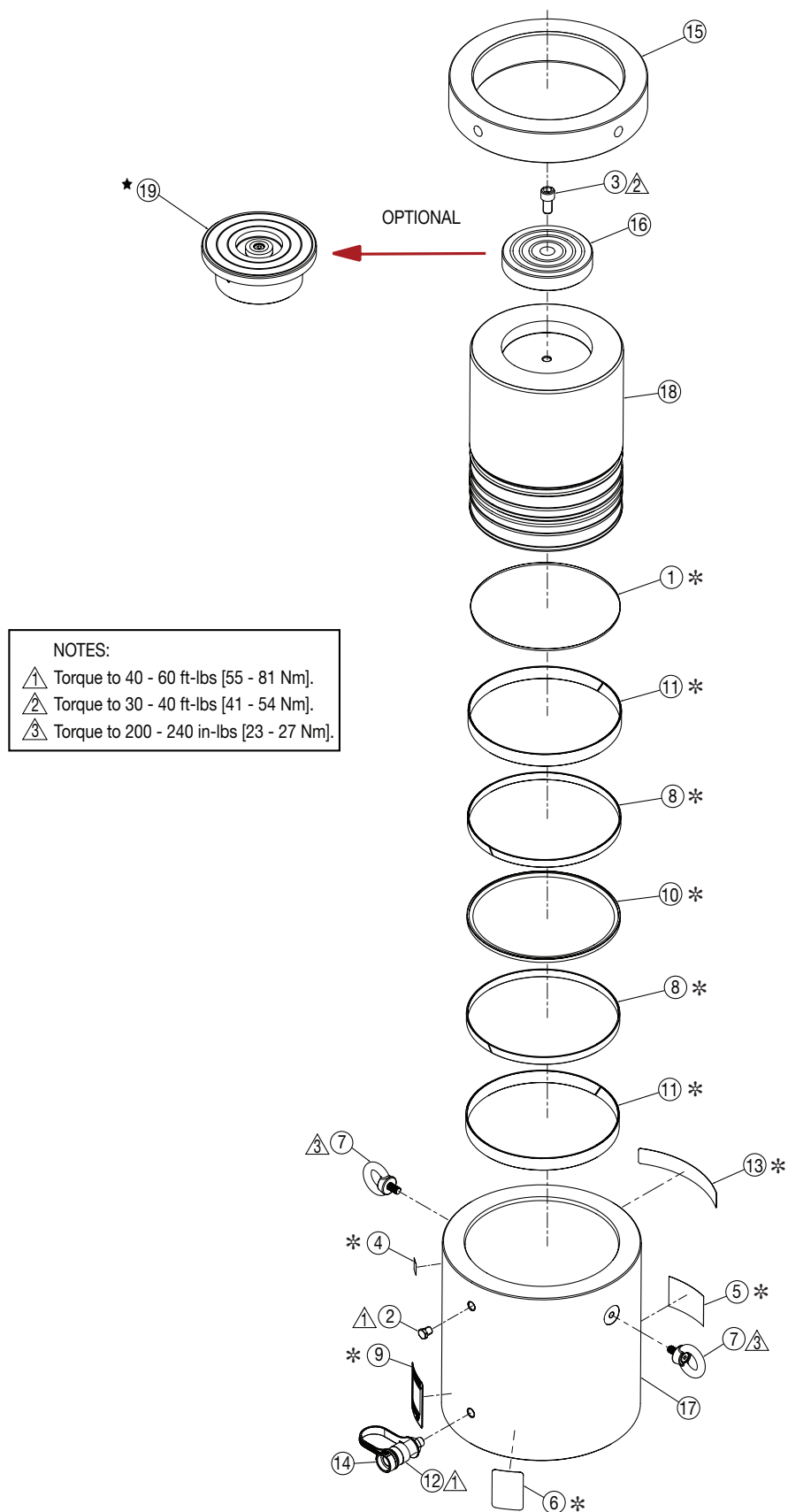
Figure 3, Exploded View - Model HCL-400
