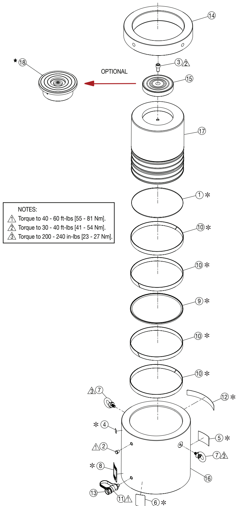
Figure 4, Exploded View - Model HCL-500
