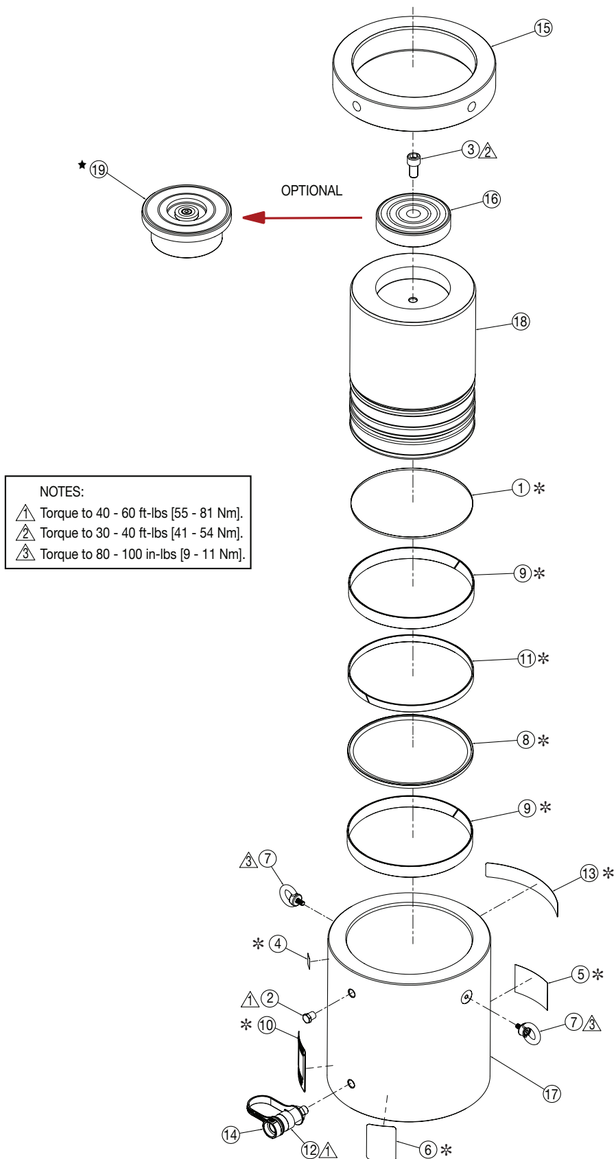
Figure 2, Exploded View - Model HCL-300
