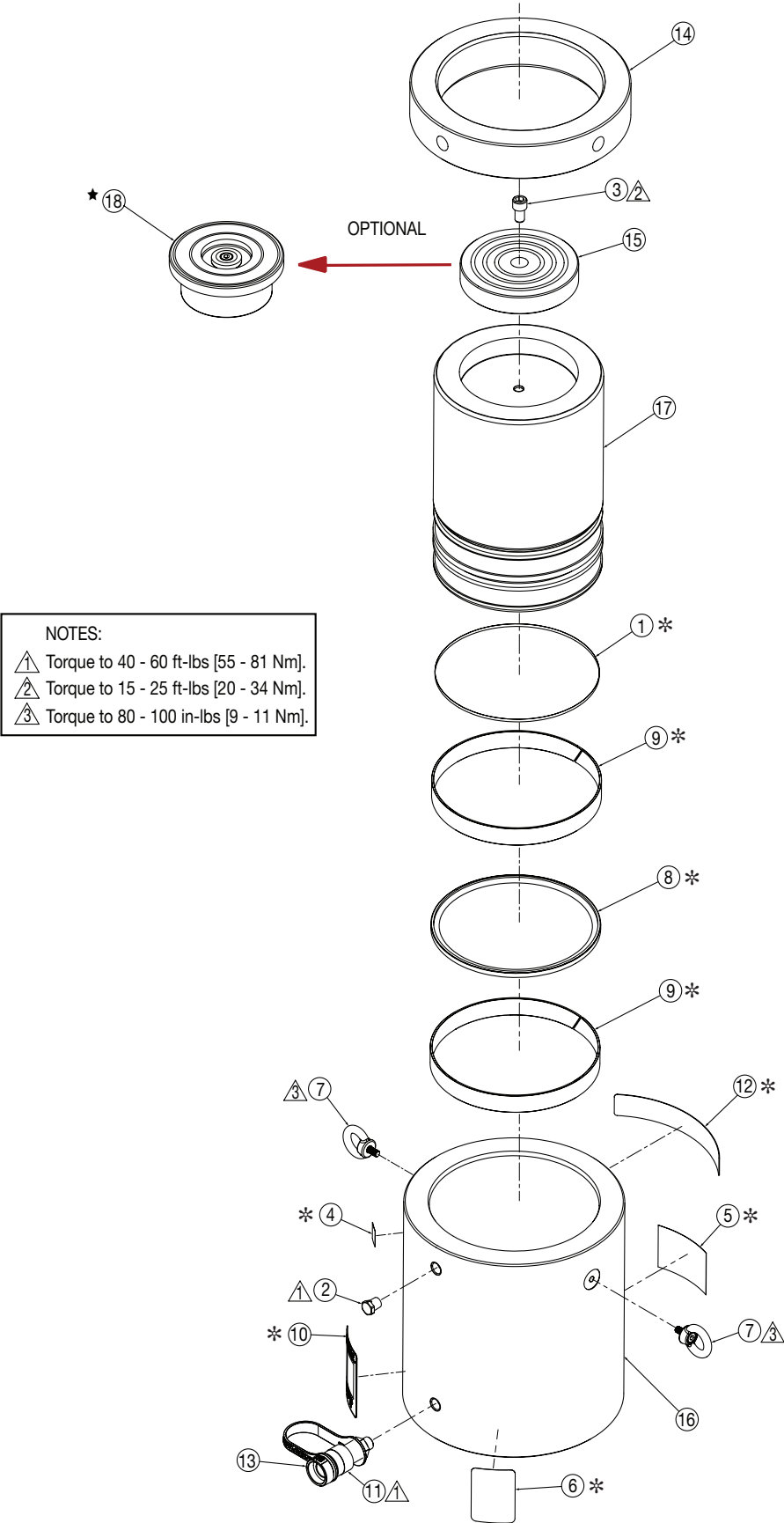
Figure 1, Exploded View - Model HCL-250
