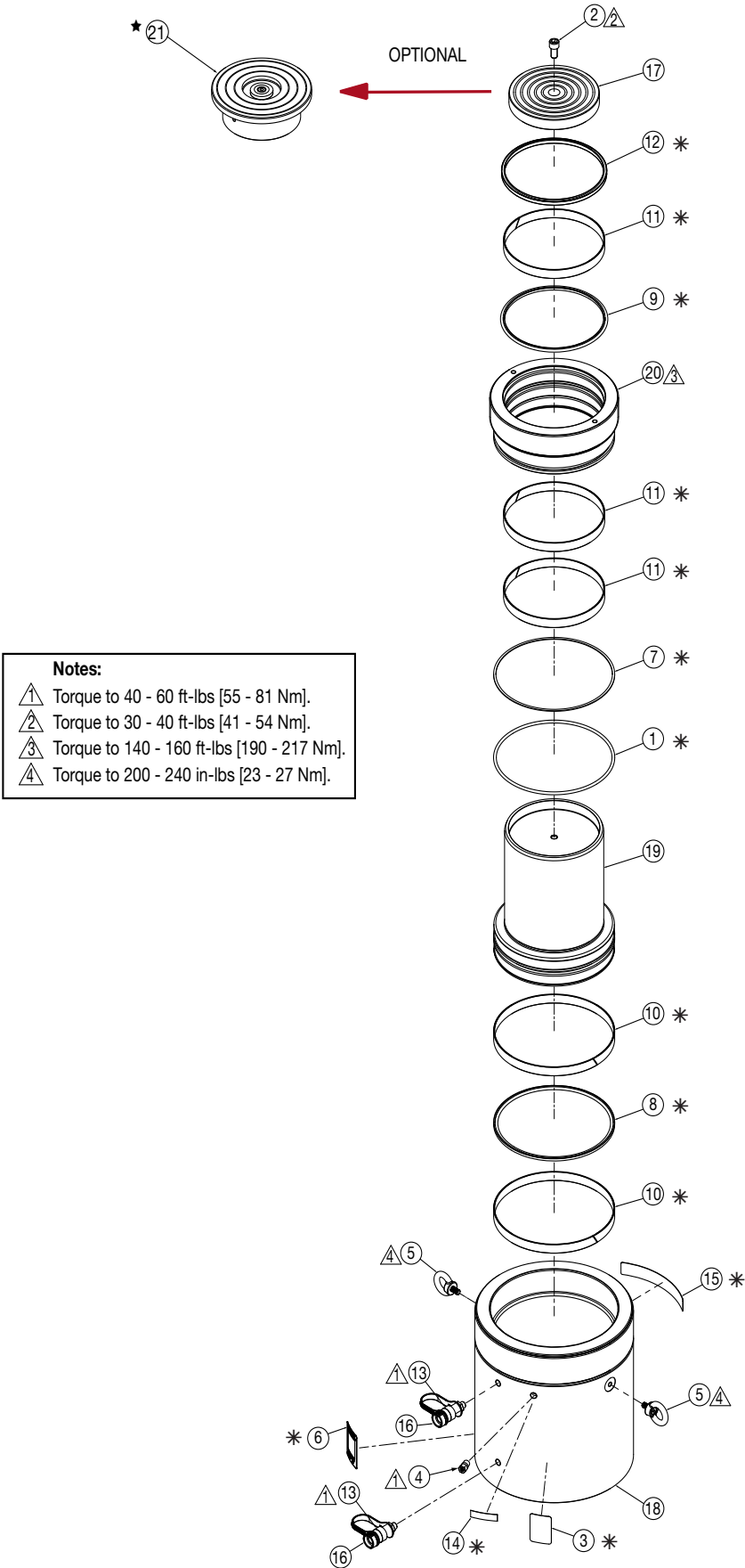
Figure 1, Exploded View - Model HCR-500
