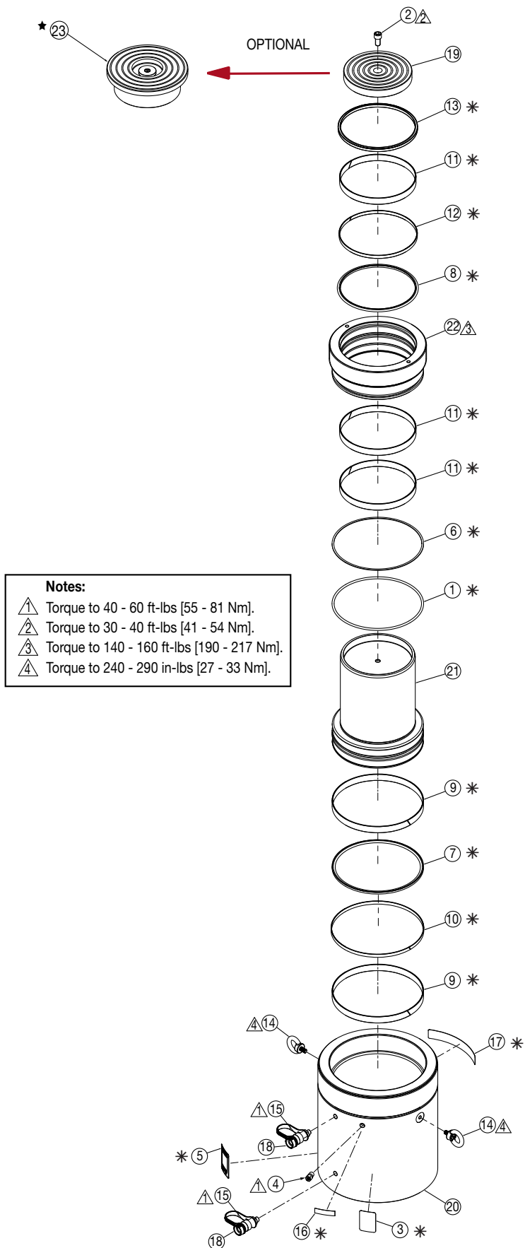
Figure 3, Exploded View - Model HCR-800
