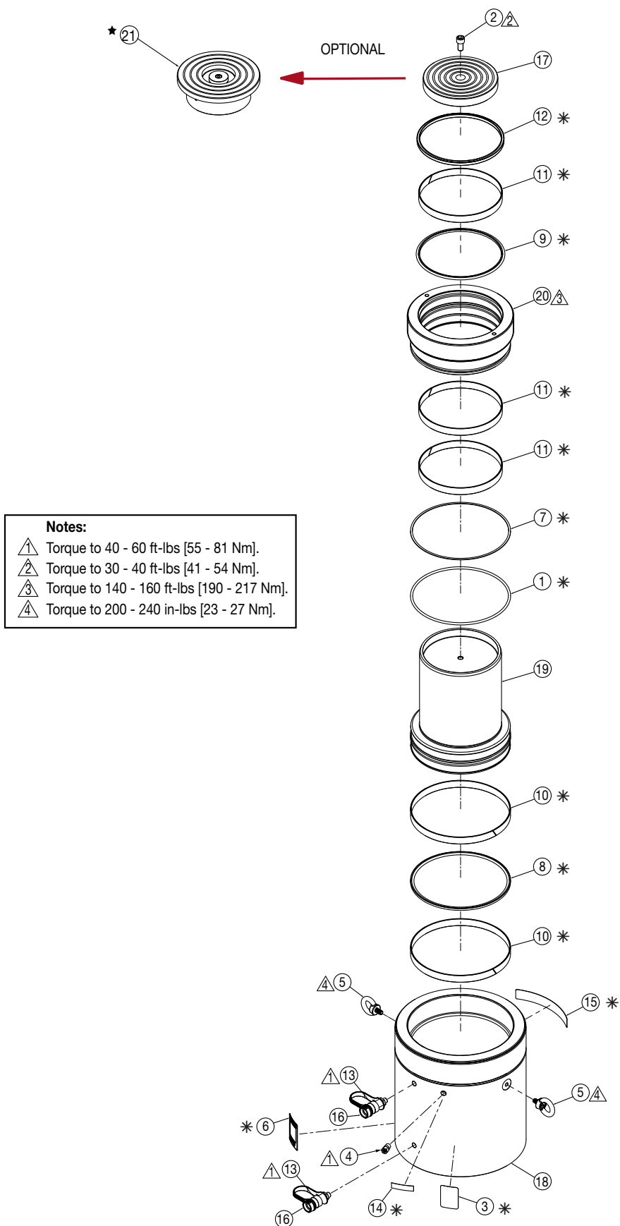
Figure 2, Exploded View - Model HCR-600
