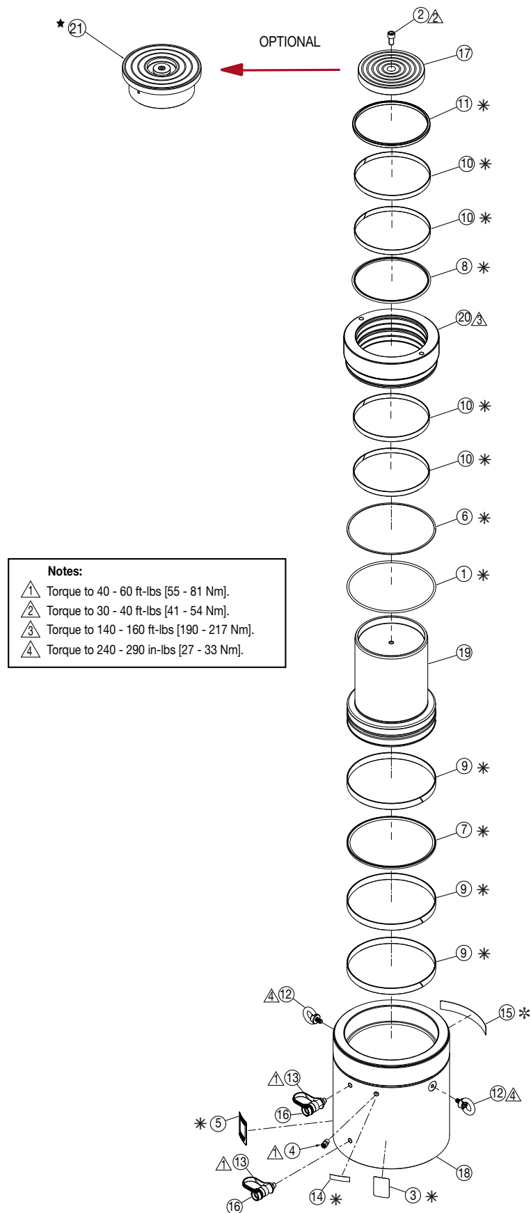
Figure 4, Exploded View - Model HCR-1000
