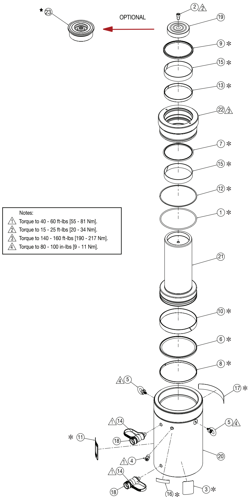
Figure 4, Exploded View - Model HCR-200 Tall
