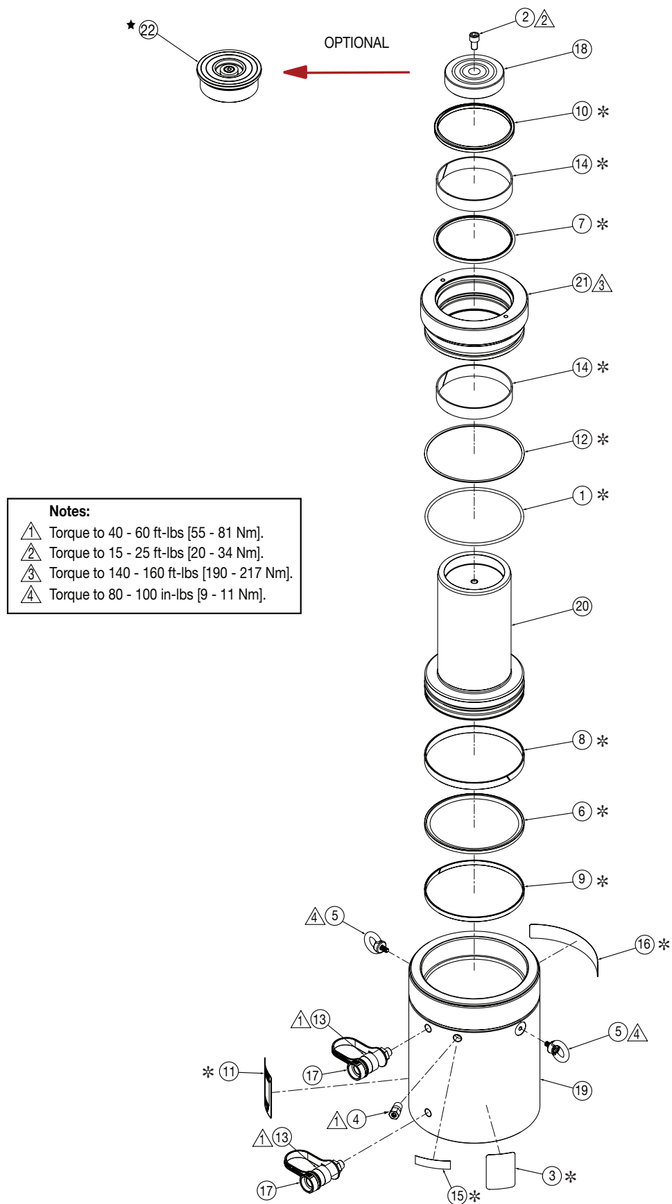
Figure 3, Exploded View - Model HCR-200 Short
