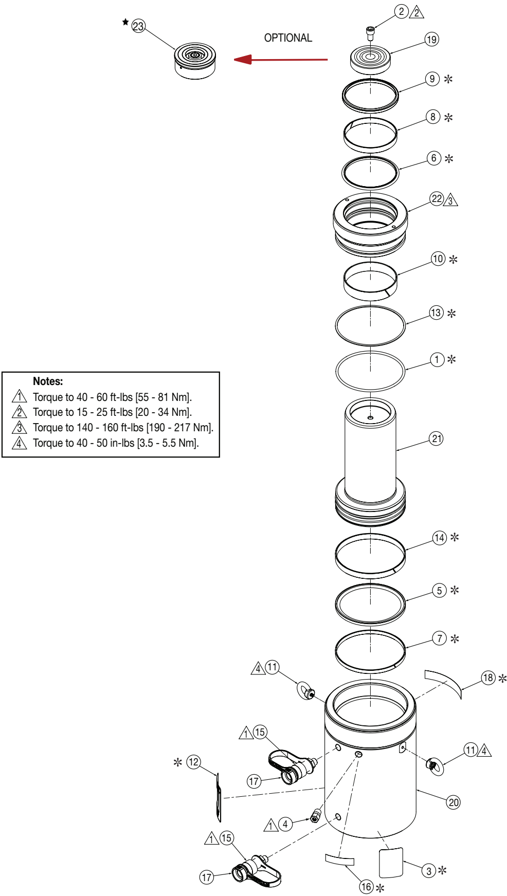
Figure 1, Exploded View - Model HCR-150 Short
