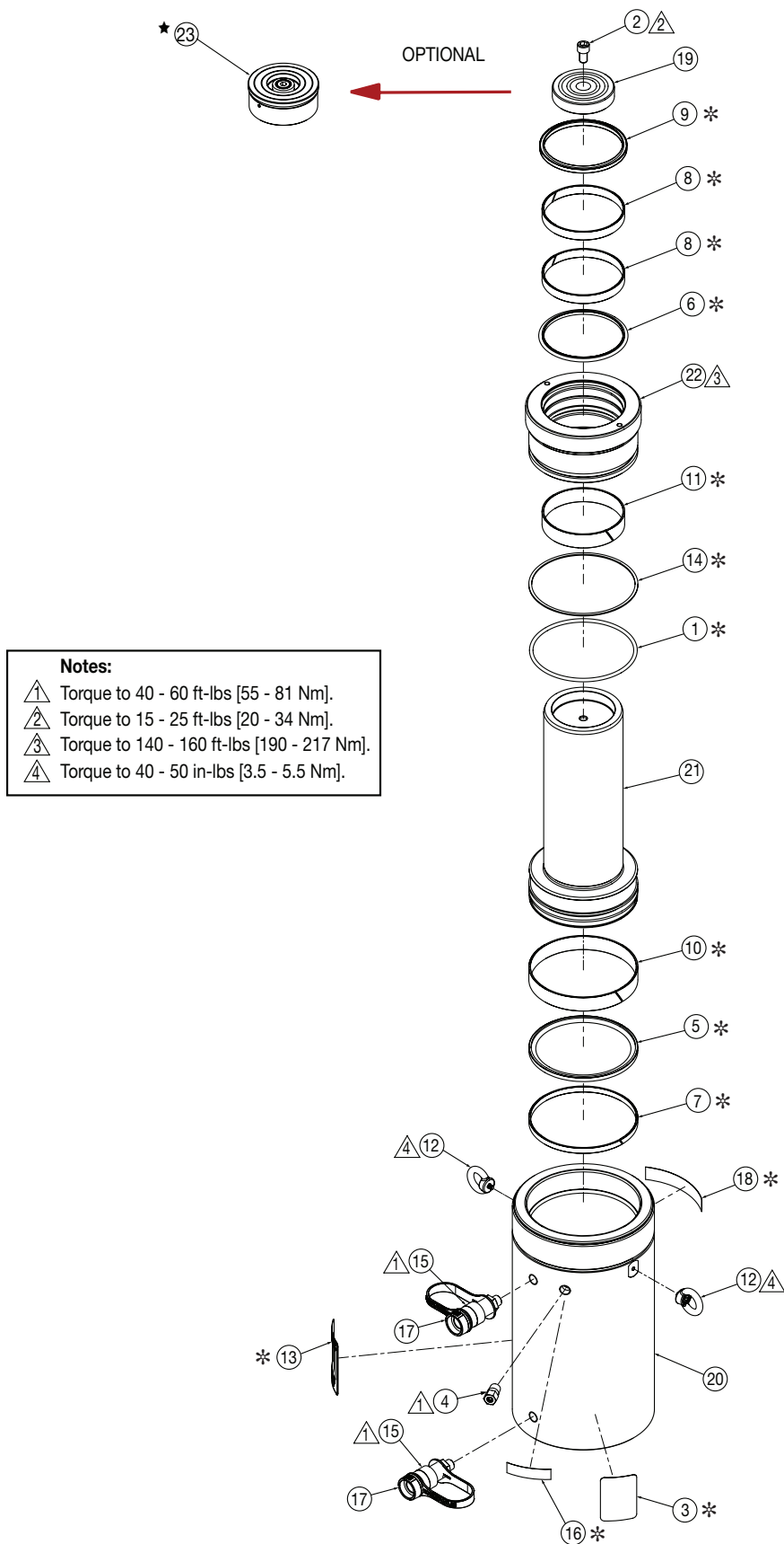
Figure 2, Exploded View - Model HCR-150 Tall
