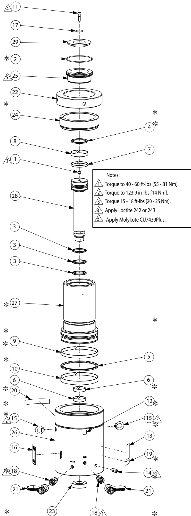
Figure 1, Exploded View - Model HCRL 3002-3006
