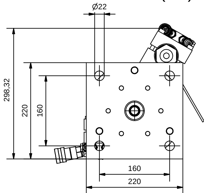
Bottom view (1:5)
