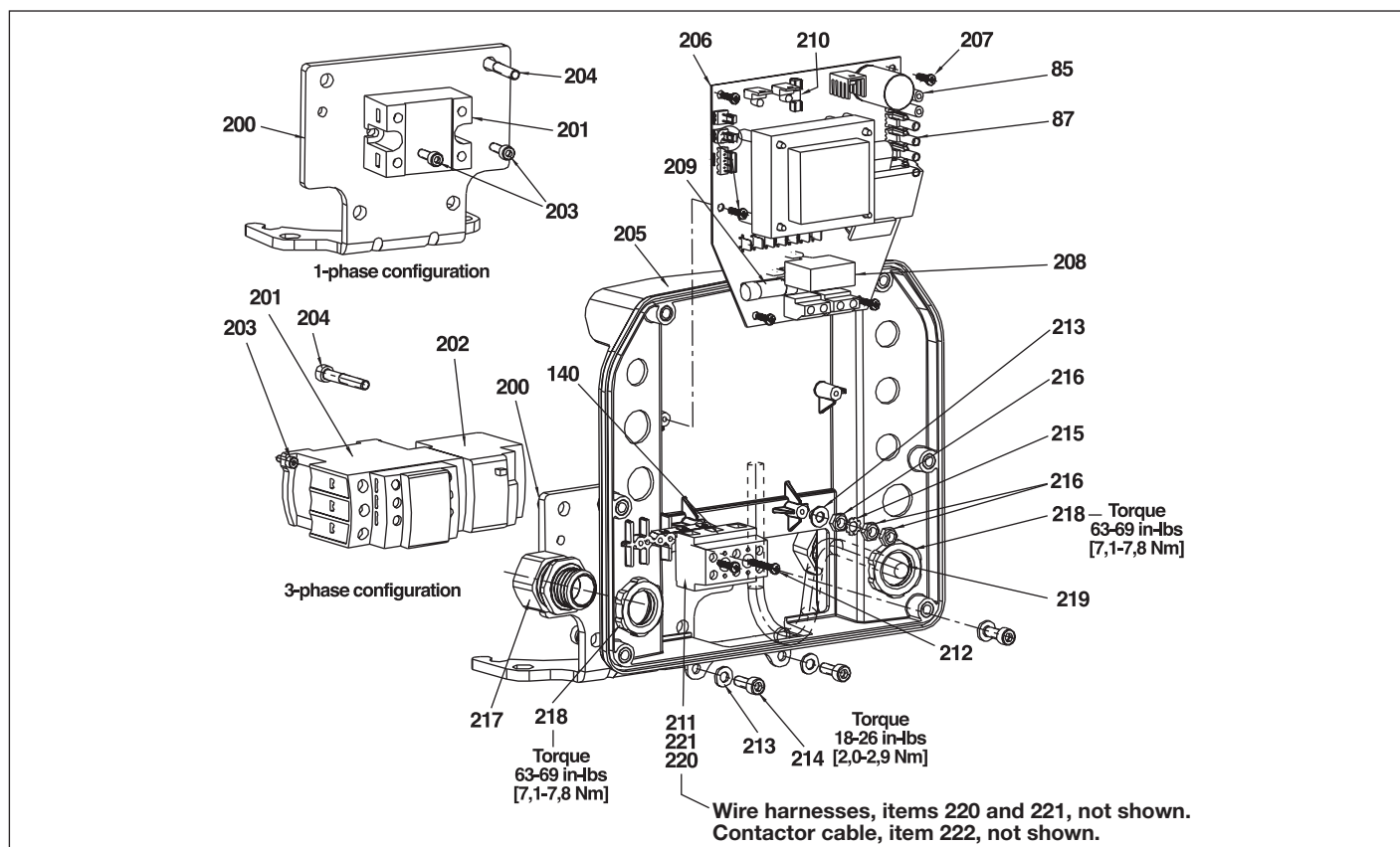
Figure 4, Rear Enclosure
