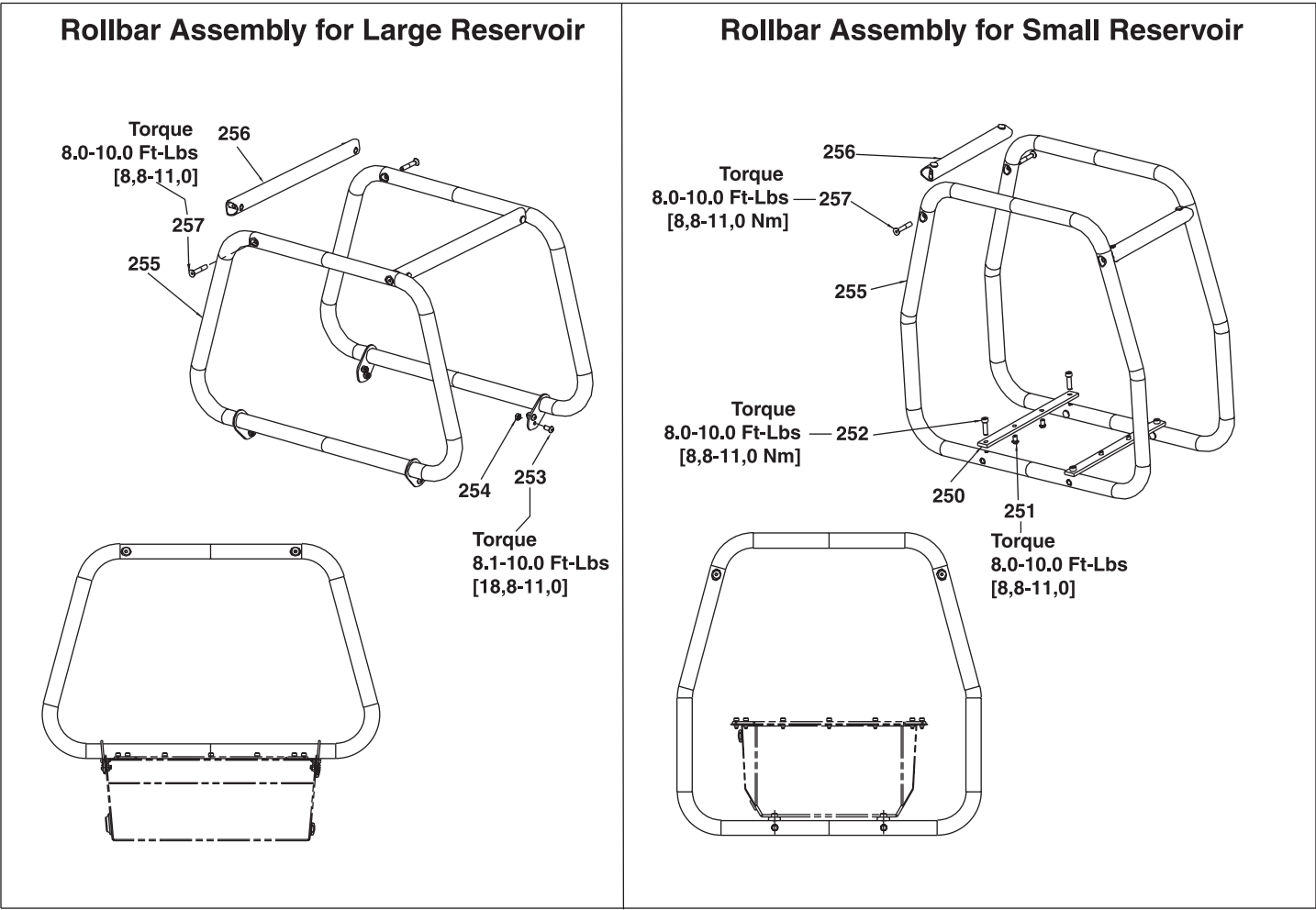
Figure 10, Rollbar Assembly
