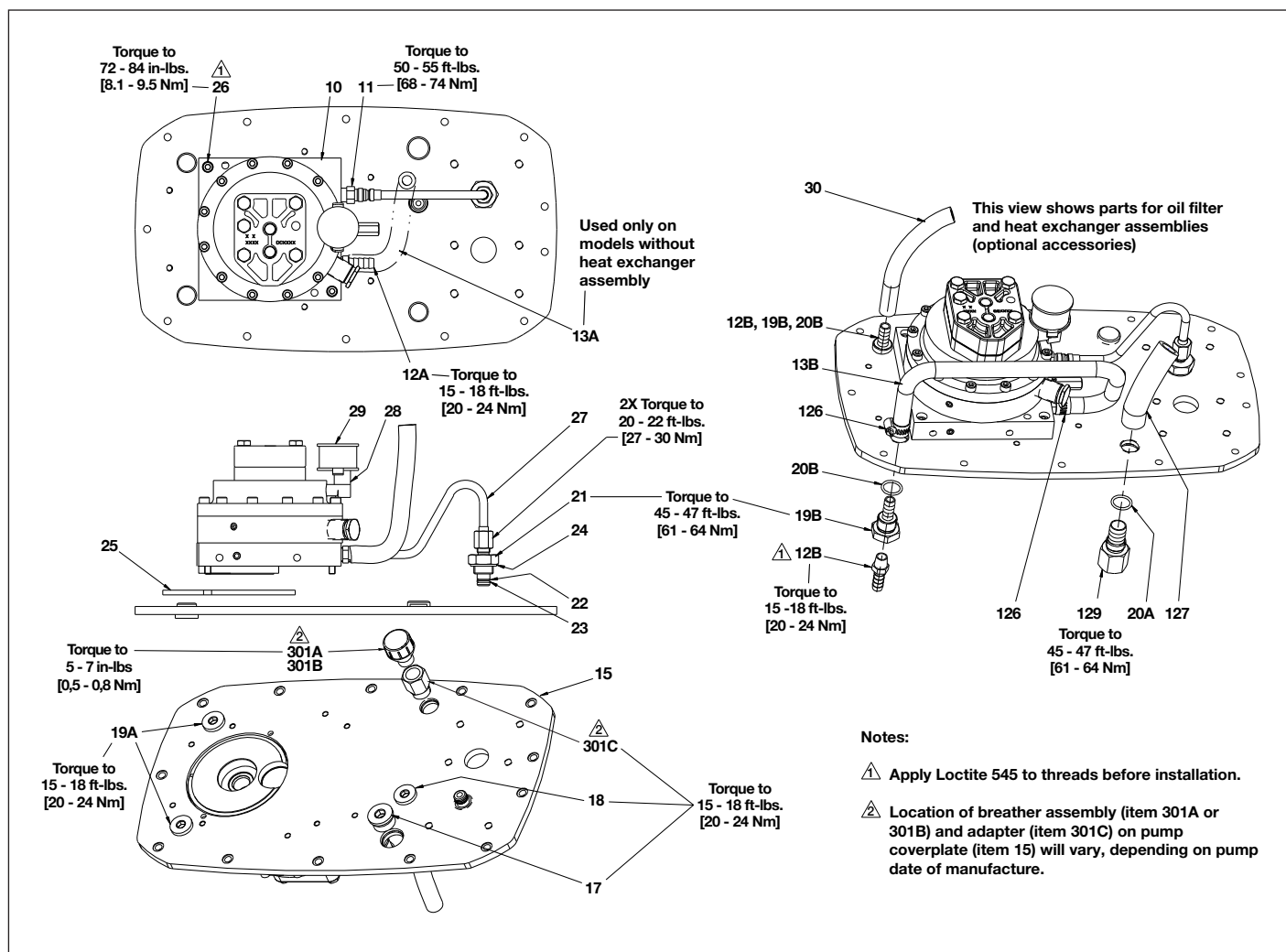
Figure 2, Basic Assembly
