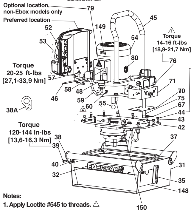
Figure 1, Pump Assembly
