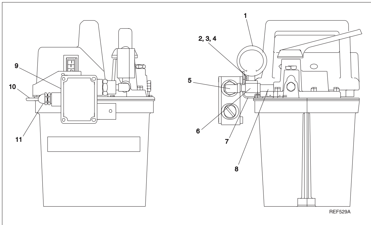
Figure 1, Pressure Switch Pumps
