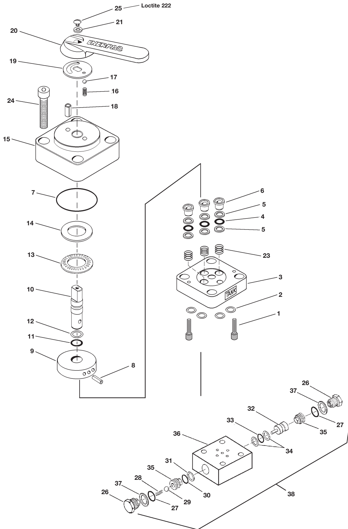
Figure 15, 3-Way Manual Valve
