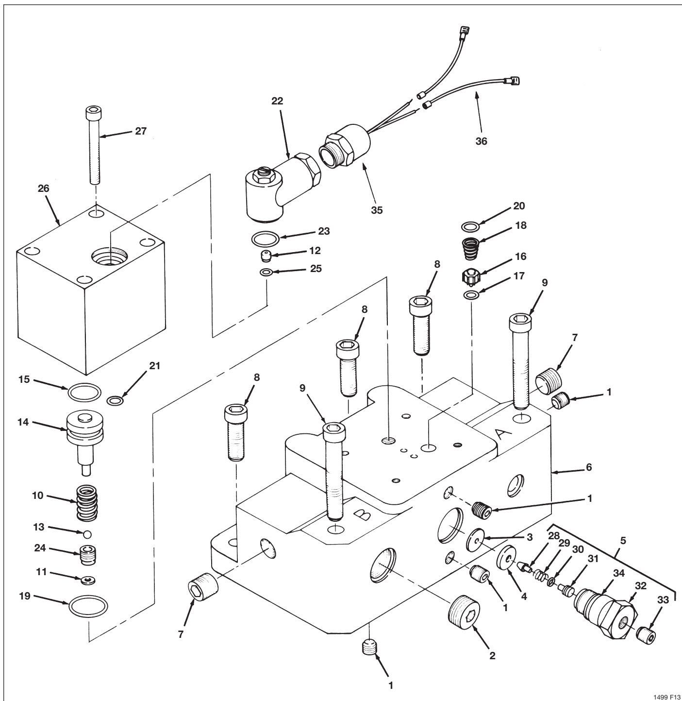
Figure 13, Dump Valve
