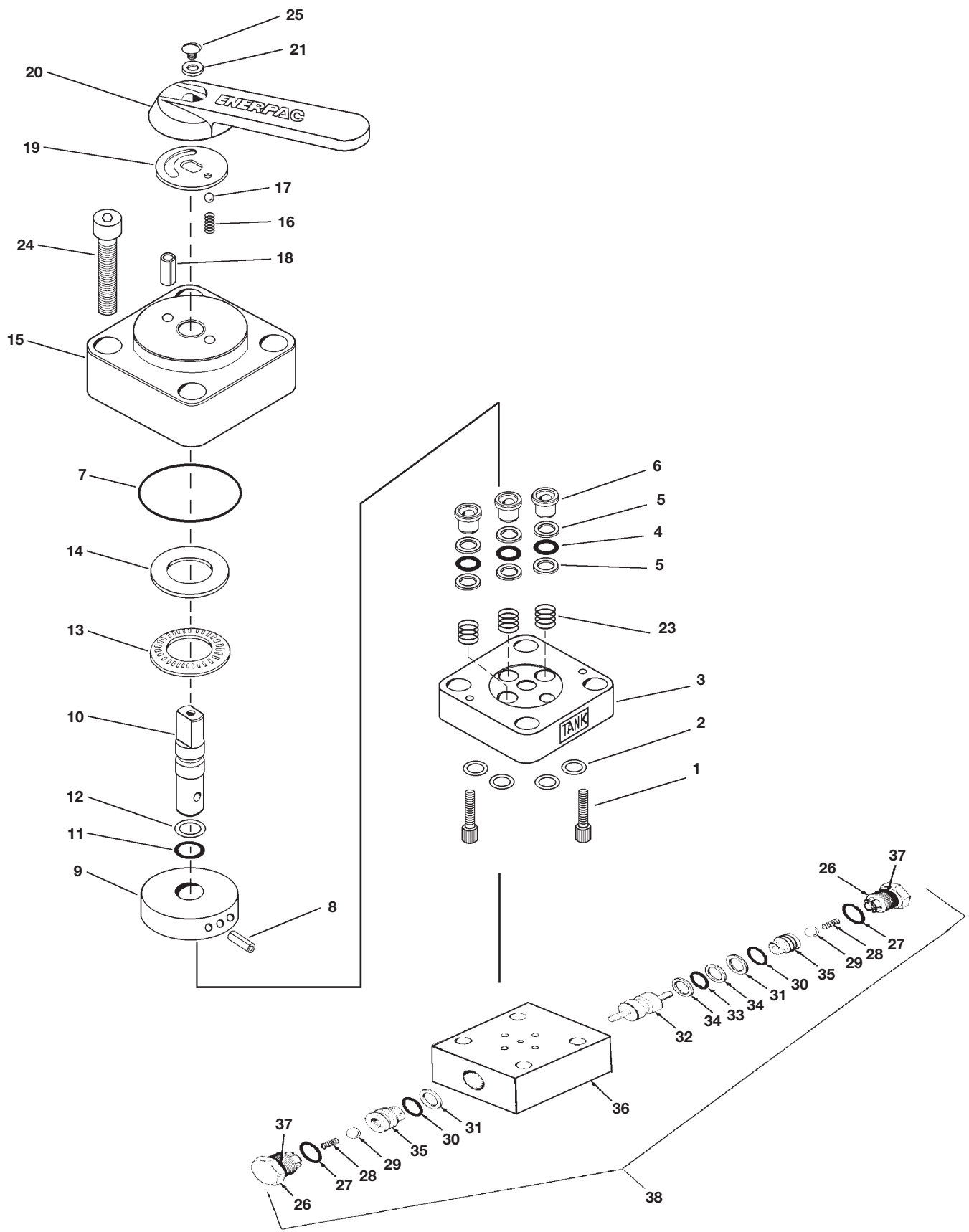
Figure 16, 4-Way Manual Valve
