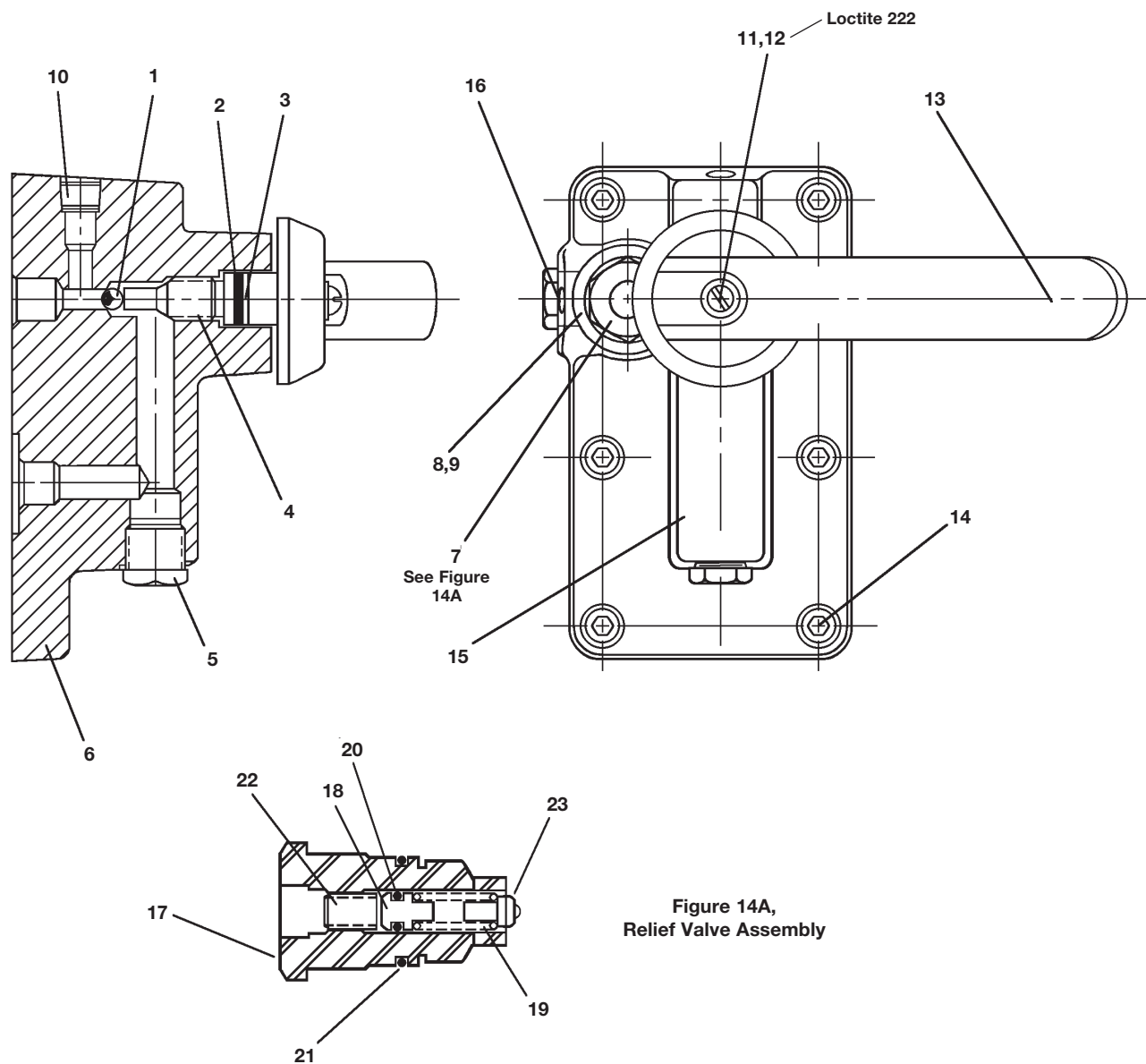
Figure 14, 2-Way Manual Valve
