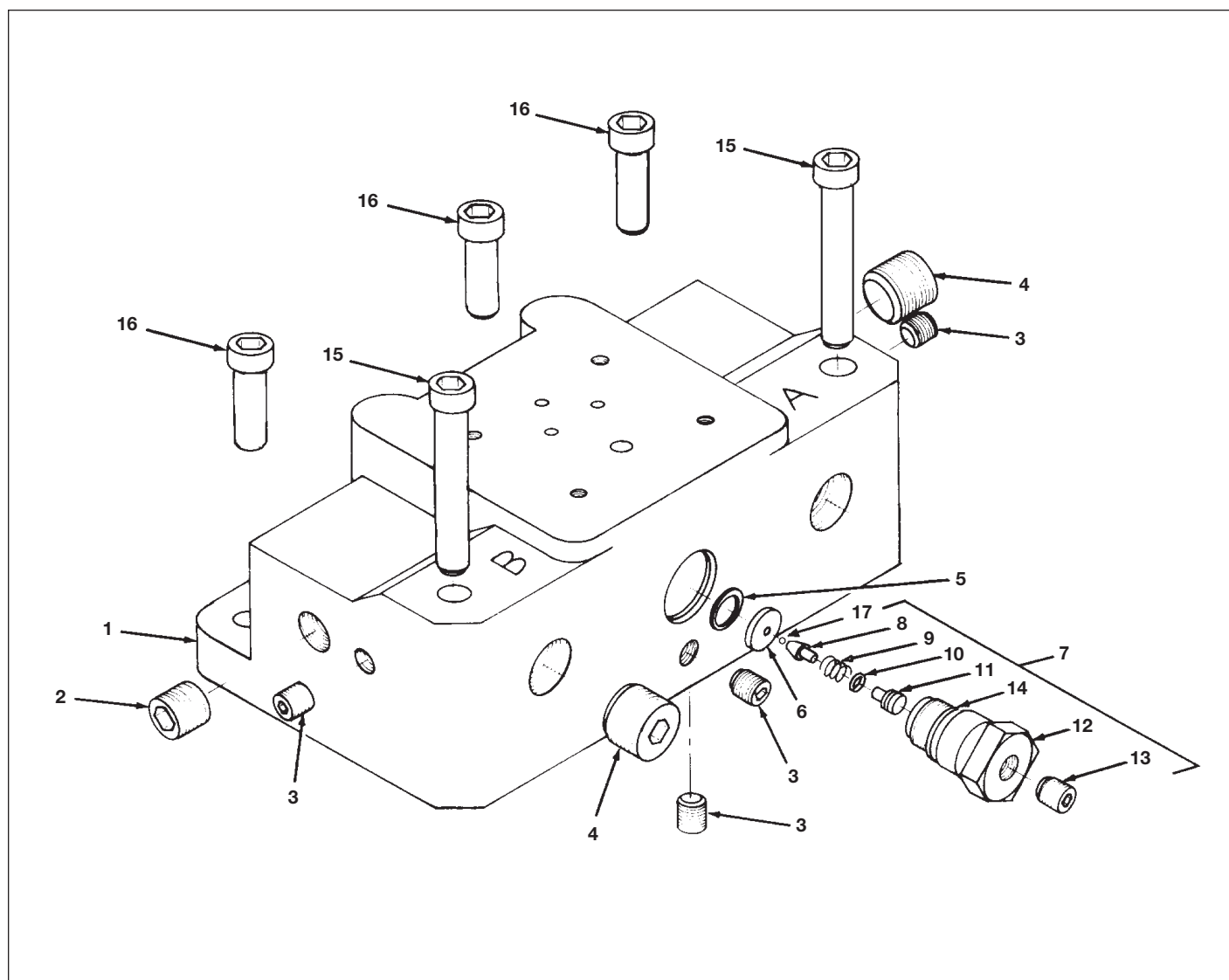
Figure 8, Pump Manifold
