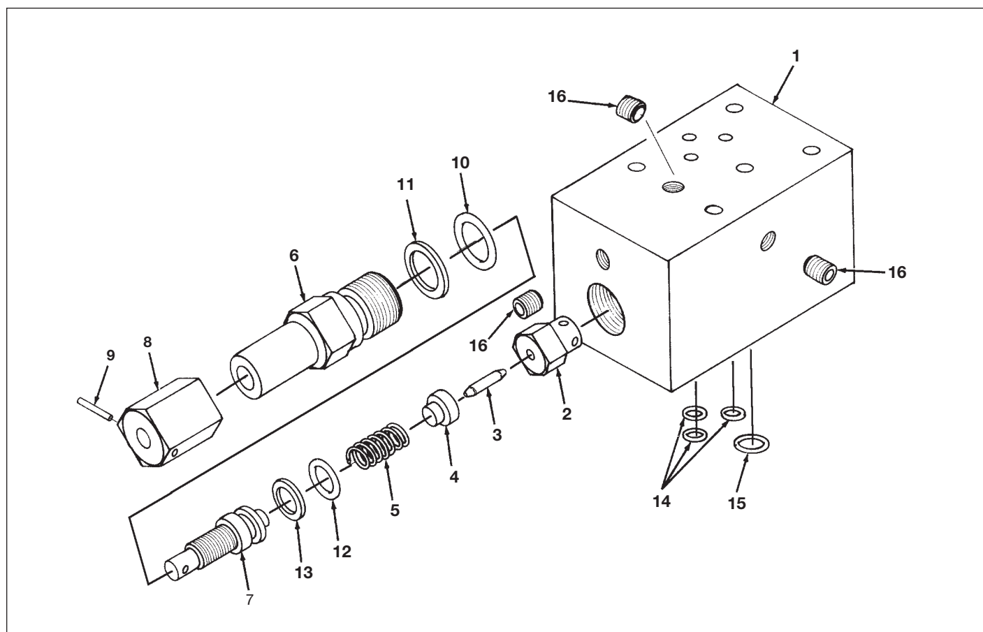
Figure 11, Relief Valve
