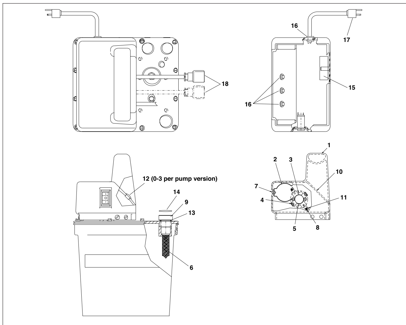
Figure 4, Shroud Assembly
