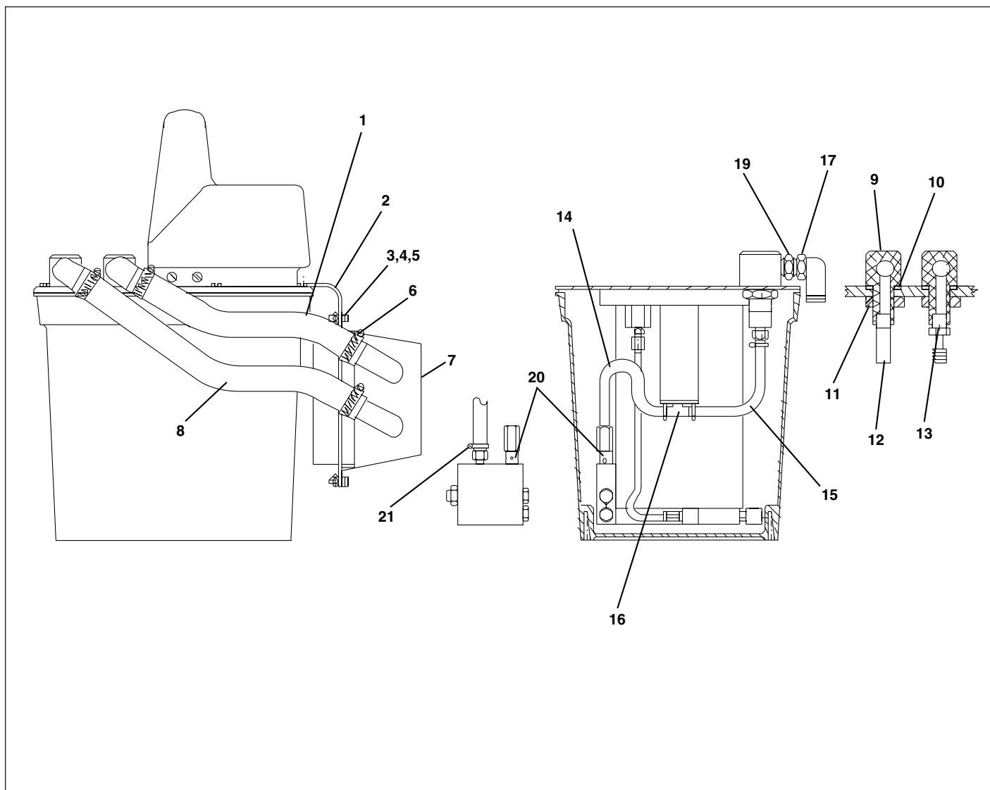
Figure 5, Heat Exchanger
