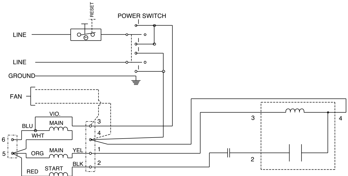
Wiring Diagram H
