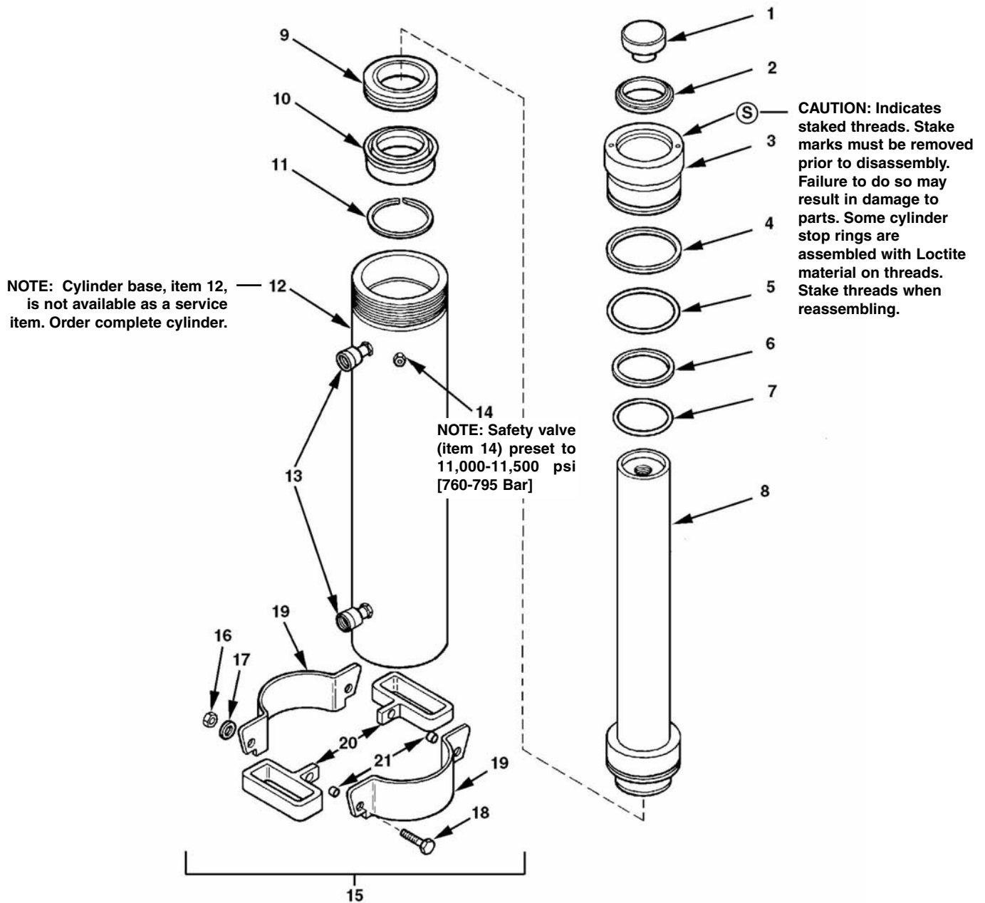
Figure 1, 100-ton, Double Acting, Solid Plunger Hydraulic Cylinders
