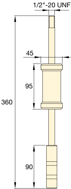
Slide Hammer Dimensions (mm)
