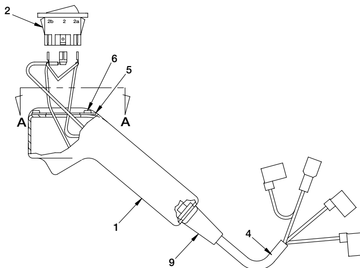
Figure 14, Pendant Assembly
