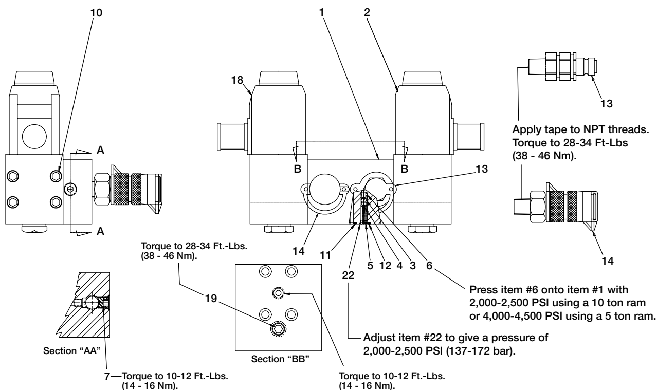
Figure 15, Poppet Valve
