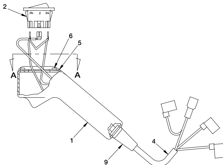
Figure 14, Pupitre mobile
