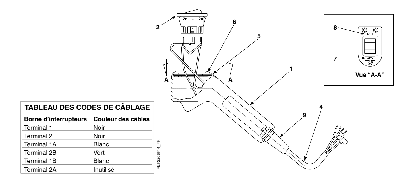
Figure 15, Pupitre mobile
