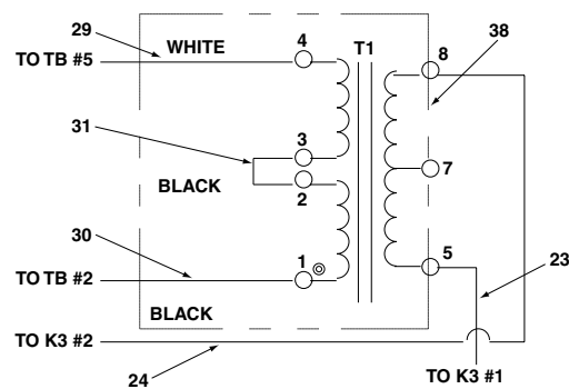
Figure 8, Wiring Diagram (Note: See pump wiring chart on next page.)
