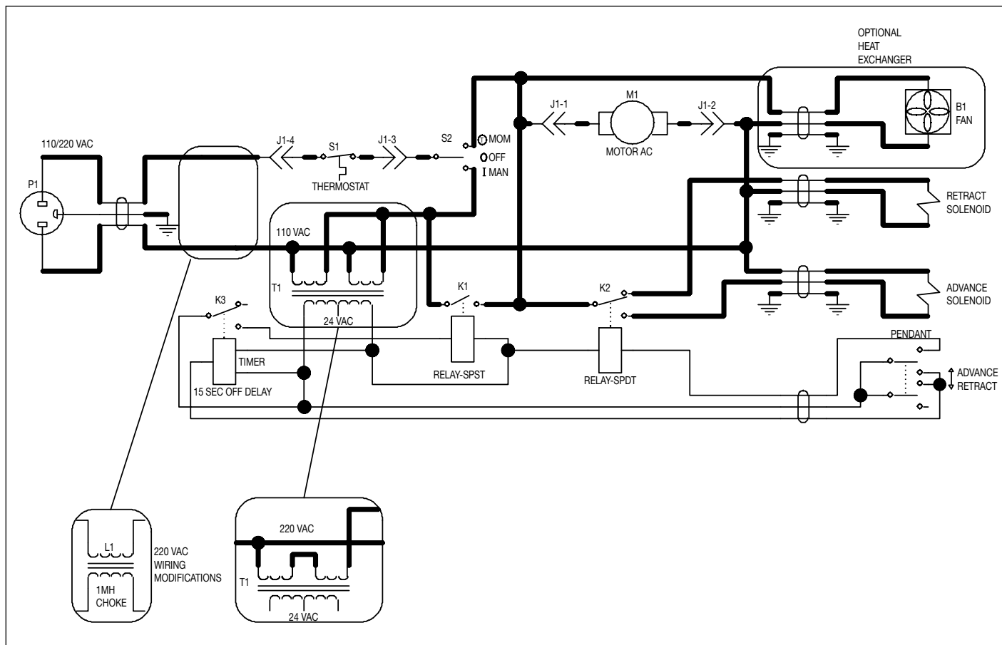
Figure 20, Electrical Schematic
