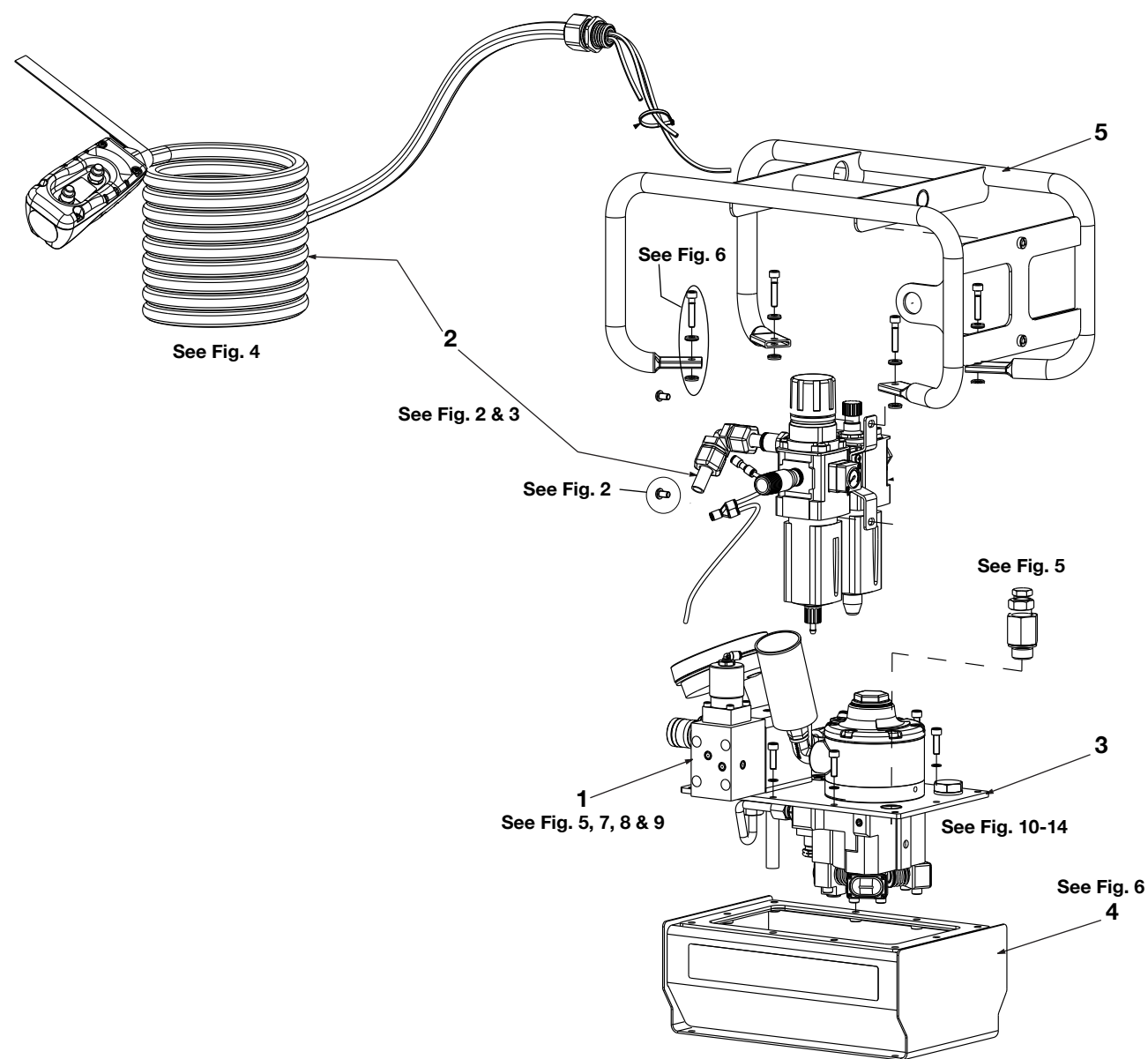
Figure 1: Main Assembly
