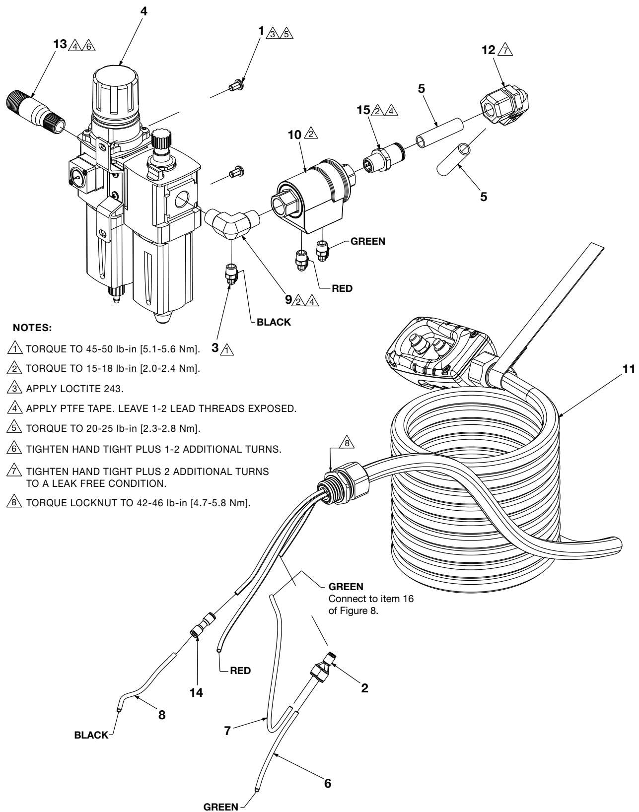
Figure 2: Filter/Regulator, Air Lubricator and Pendant Assembly
