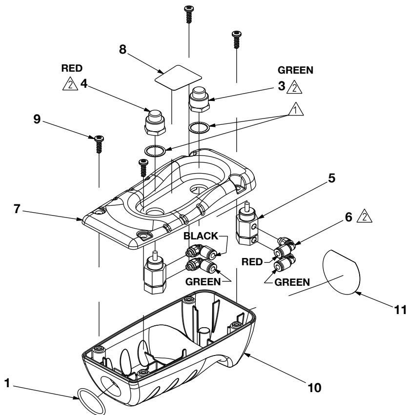
Figure 4: Air Pendant Assembly
